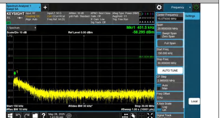
Band4-20MHz-QPSK-20050-1RB#0-0.15~30-PASS
