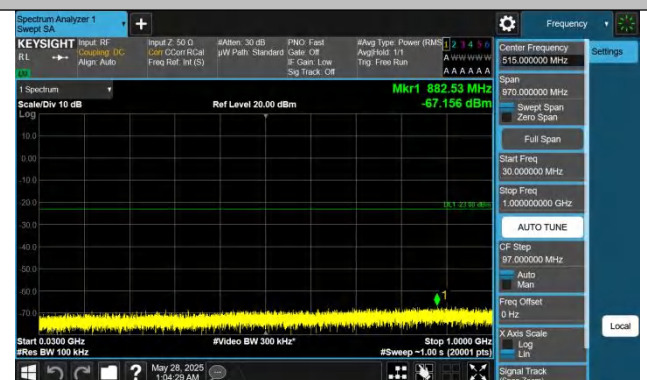
Band4-5MHz-QPSK-20375-1RB#24-30~1000-PASS
