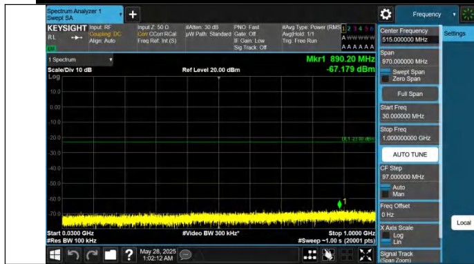
Band4-5MHz-QPSK-20175-1RB#0-30~1000-PASS
