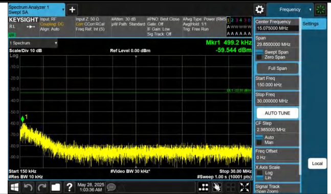
Band4-5MHz-QPSK-20375-1RB#0-0.15~30-PASS
