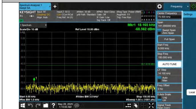
Band4-10MHz-QPSK-20000-1RB#0-0.009~0.15-PASS
