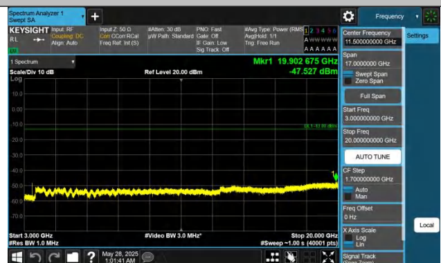
Band4-5MHz-QPSK-19975-1RB#24-3000~20000-PASS
