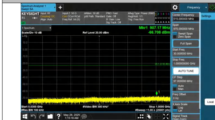
Band4-10MHz-QPSK-20000-1RB#0-30~1000-PASS
