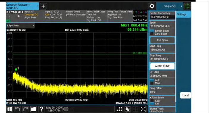
Band4-15MHz-QPSK-20025-1RB#0-0.15~30-PASS
