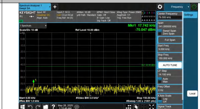
Band4-10MHz-QPSK-20000-1RB#49-0.009~0.15-PASS
