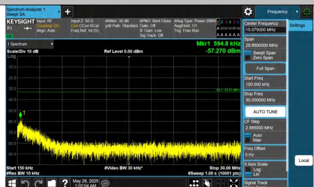
Band4-5MHz-QPSK-20175-1RB#0-0.15~30-PASS
