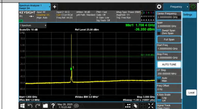
Band4-10MHz-QPSK-20000-1RB#0-1000~3000-PASS
