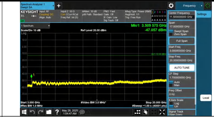
Band4-5MHz-QPSK-20375-1RB#24-3000~20000-PASS
