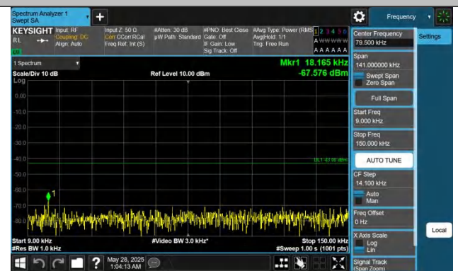
Band4-5MHz-QPSK-20375-1RB#24-0.009~0.15-PASS
