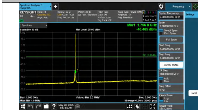
Band4-20MHz-QPSK-20300-1RB#99-1000~3000-PASS
