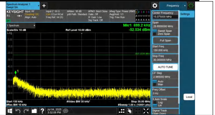
Band5-4233-1-0.15~30MHz-PASS
