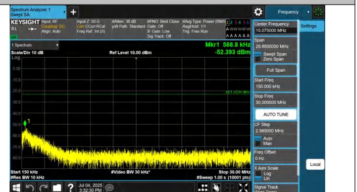
Band5-4132-2-0.15~30MHz-PASS
