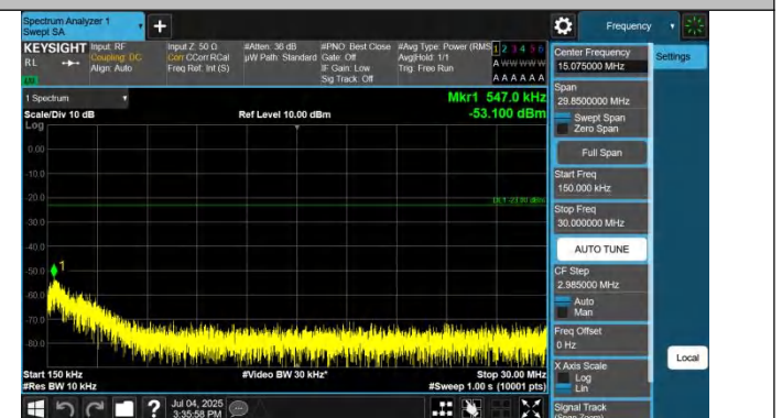
Band5-4182-5-0.15~30MHz-PASS
