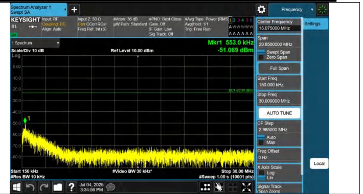
Band5-4182-4-0.15~30MHz-PASS
