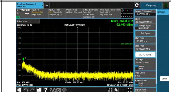
Band5-4182-4-0.15~30MHz-PASS
