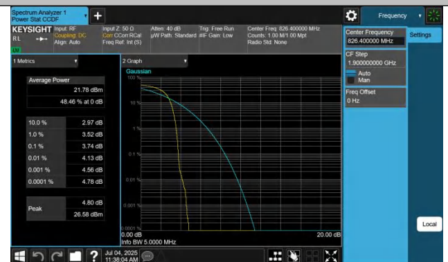
Band5-4132-4-PASS
