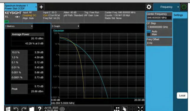
Band5-4233-4-PASS
