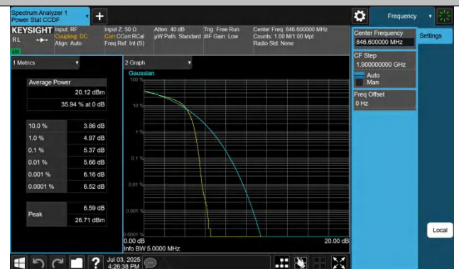
Band5-4233-2-PASS
