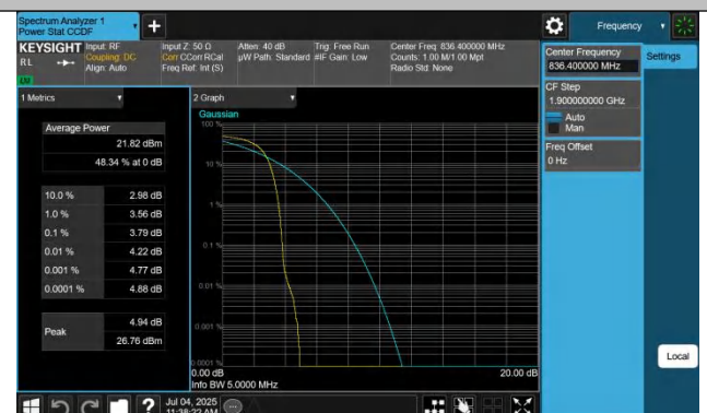
Band5-4182-4-PASS
