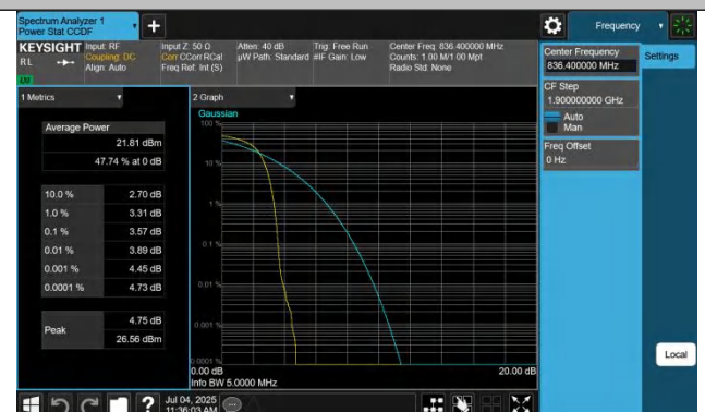
Band5-4182-2-PASS
