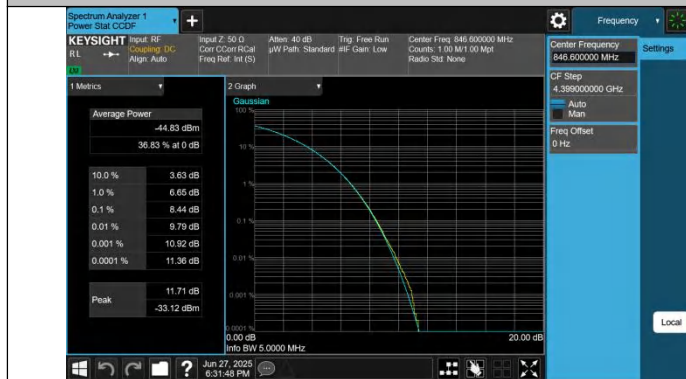
Band5-4233-PASS
