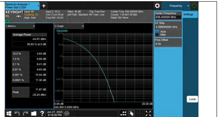
Band5-4182-PASS
