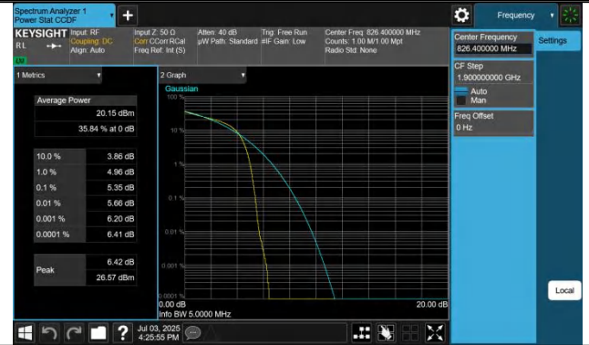
Band5-4132-2-PASS
