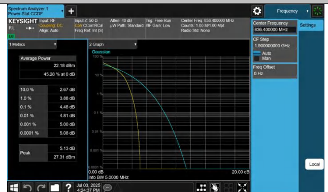
Band5-4182-1-PASS
