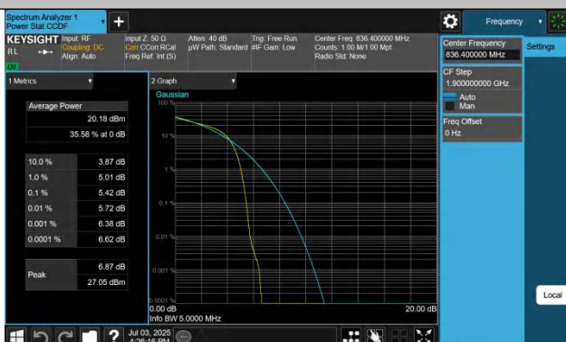
Band5-4182-2-PASS
