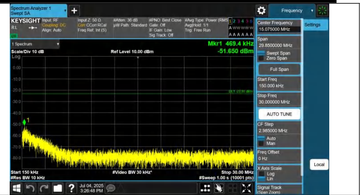
Band5-4233-0.15~30MHz-PASS
