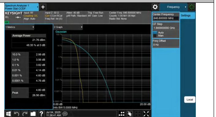
Band5-4233-4-PASS
