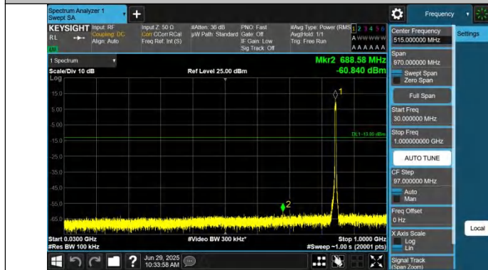
Band5-4233-30~1000MHz-PASS
