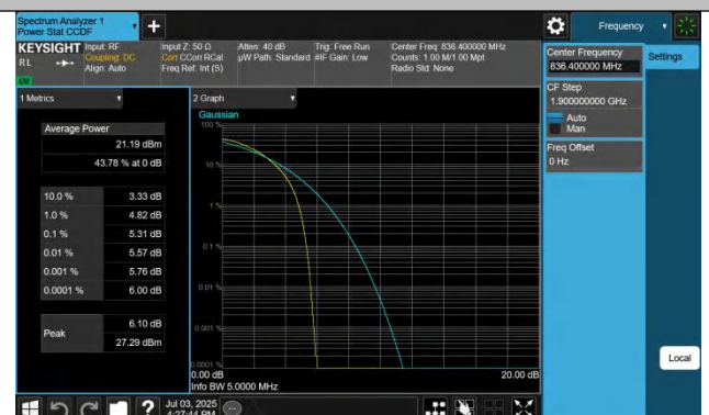
Band5-4182-3-PASS
