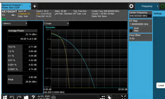
Band5-4233-5-PASS
