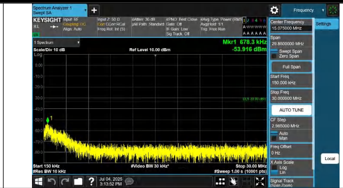
Band2-9400-2-0.15~30MHz-PASS
