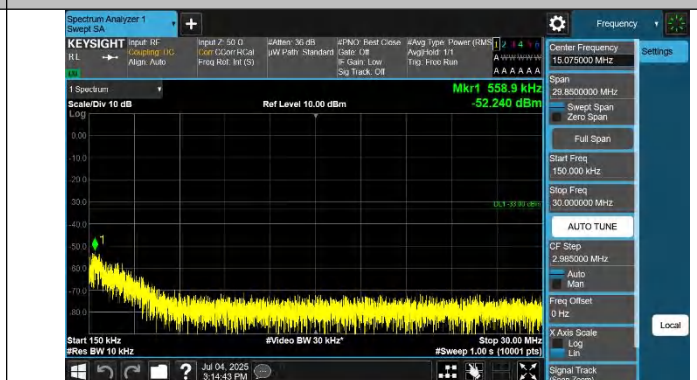
Band2-9538-3-0.15~30MHz-PASS
