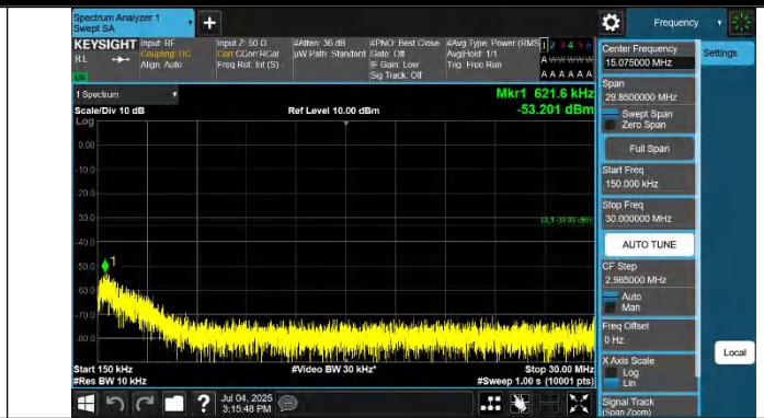
Band2-9400-1-0.15~30MHz-PASS
