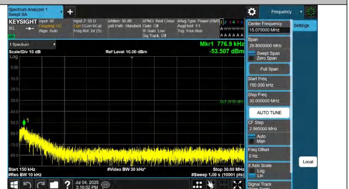
Band2-9262-3-0.15~30MHz-PASS
