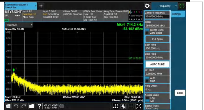
Band2-9262-2-0.15~30MHz-PASS
