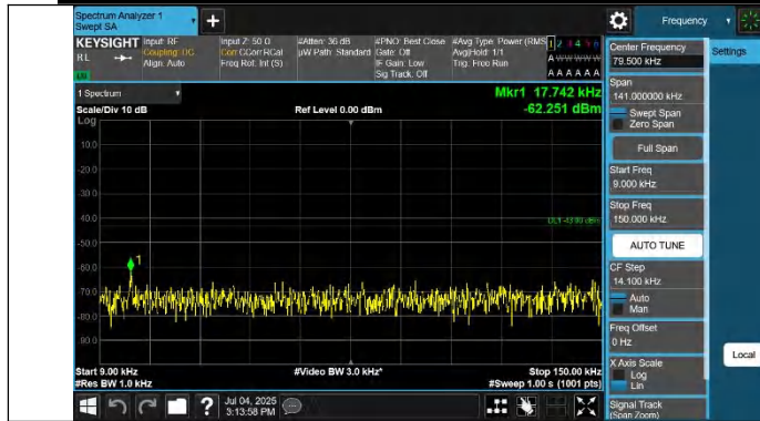
Band2-9538-2-0.009~0.15MHz-PASS
