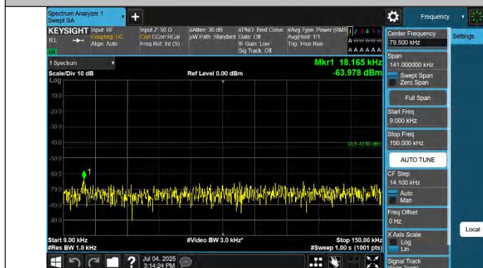
Band2-9400-3-0.009~0.15MHz-PASS
