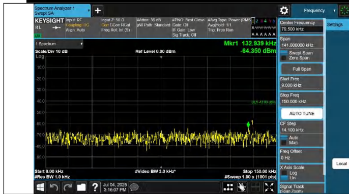
Band2-9262-2-0.009~0.15MHz-PASS
