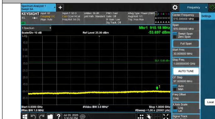
Band2-9262-3-30~1000MHz-PASS
