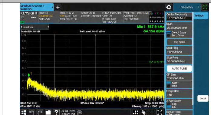
Band2-9400-2-0.15~30MHz-PASS
