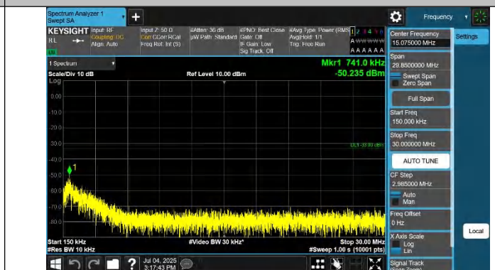
Band2-9400-4-0.15~30MHz-PASS
