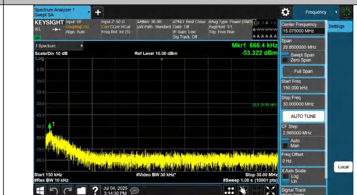
Band2-9400-3-0.15~30MHz-PASS
