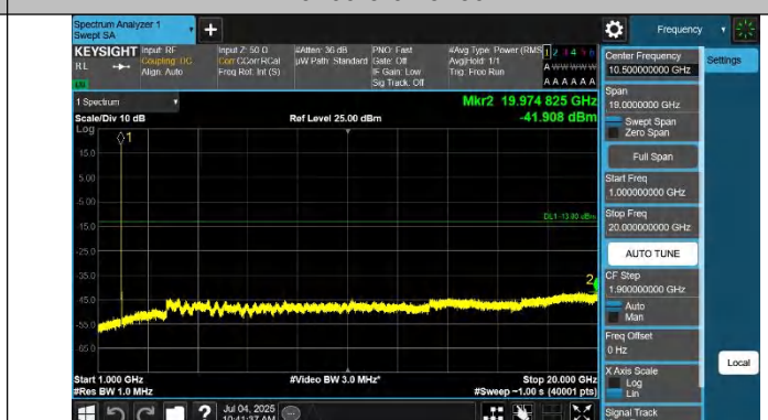
Band2-9400-3-1000~20000MHz-PASS
