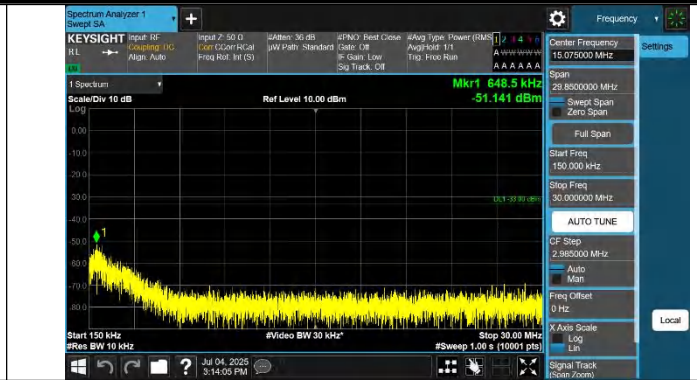
Band2-9538-2-0.15~30MHz-PASS
