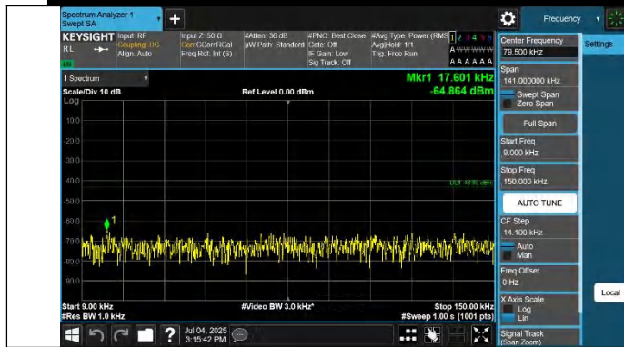
Band2-9400-1-0.009~0.15MHz-PASS
