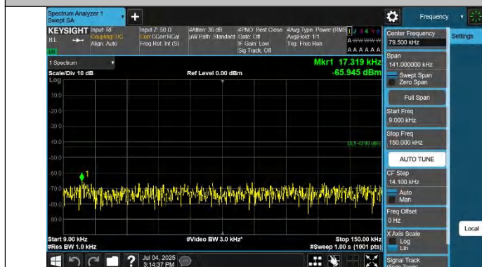
Band2-9538-3-0.009~0.15MHz-PASS
