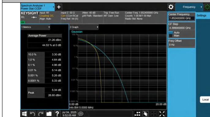
Band2-9262-3-PASS
