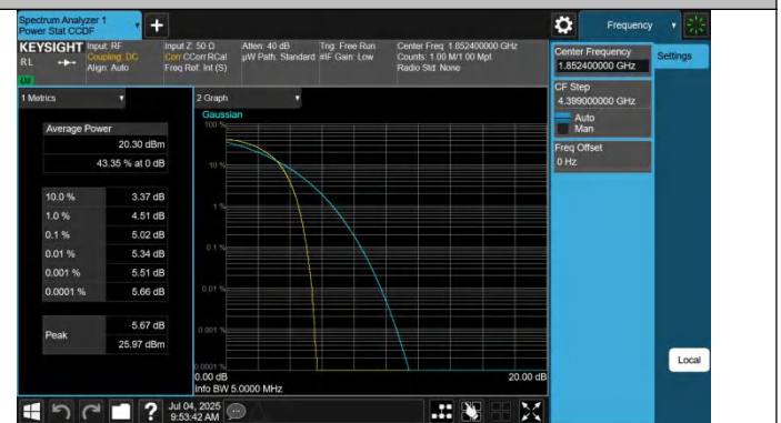
Band2-9262-4-PASS
