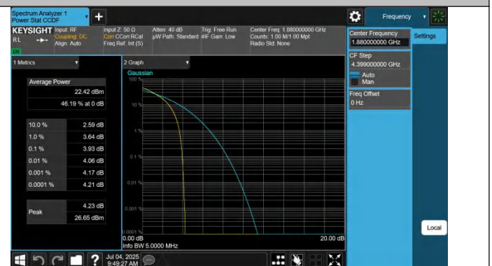
Band2-9400-1-PASS
