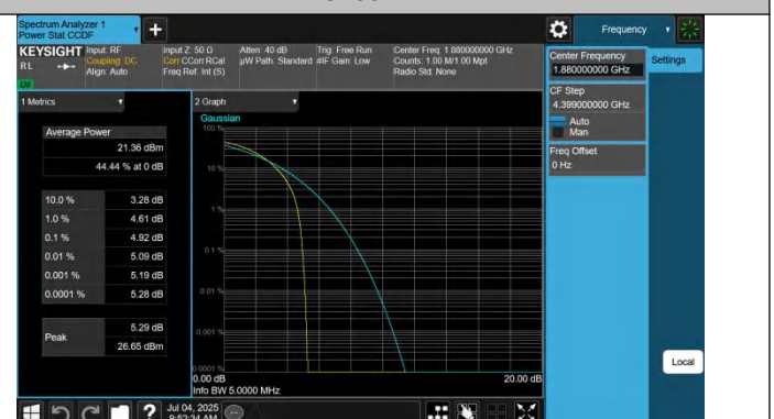
Band2-9400-3-PASS
