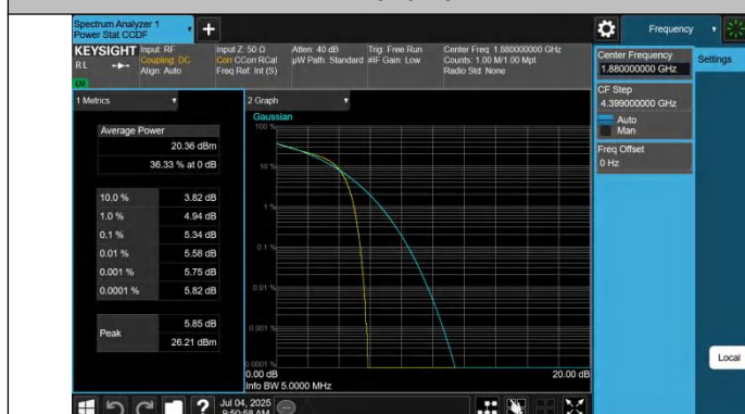
Band2-9400-2-PASS
