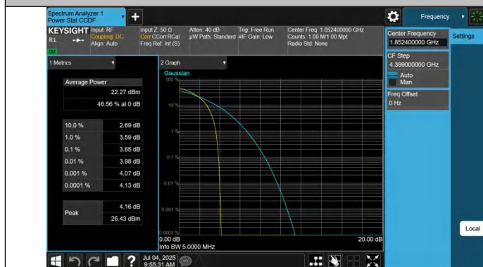
Band2-9262-5-PASS
