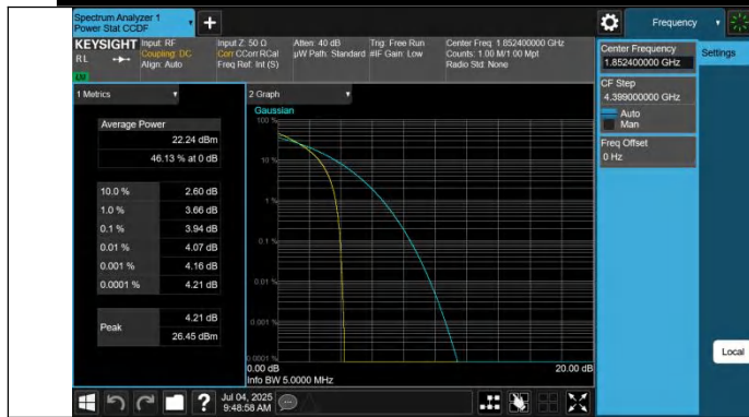
Band2-9262-1-PASS
