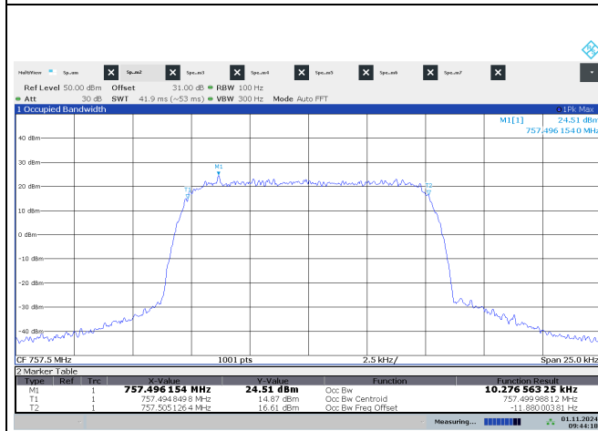
757.5 MHz_QPSK_12.5k_Port 1
