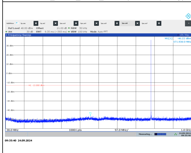
787.5 MHz_QPSK_12.5k_Port 2 (Low Frequency)
