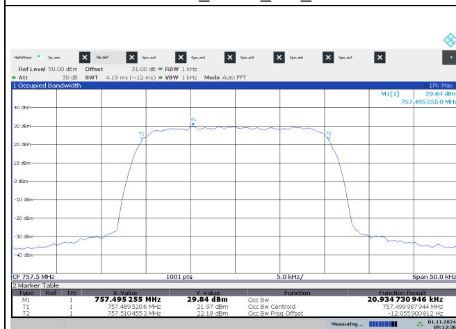
757.5 MHz_QPSK_25k_Port 1
