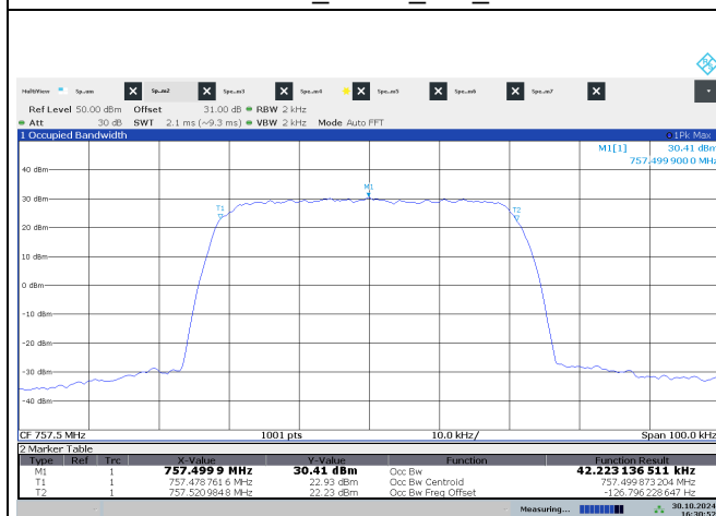
757.5 MHz_QPSK_50k_Port 1
