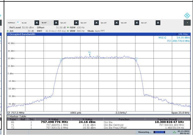
757.5 MHz_QPSK_12.5k_Port 2
