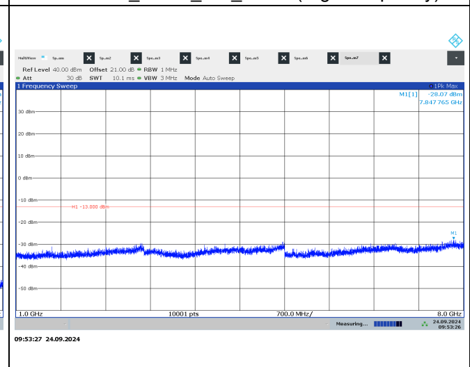
787.5 MHz_QPSK_25k_Port 1 (High Frequency)
