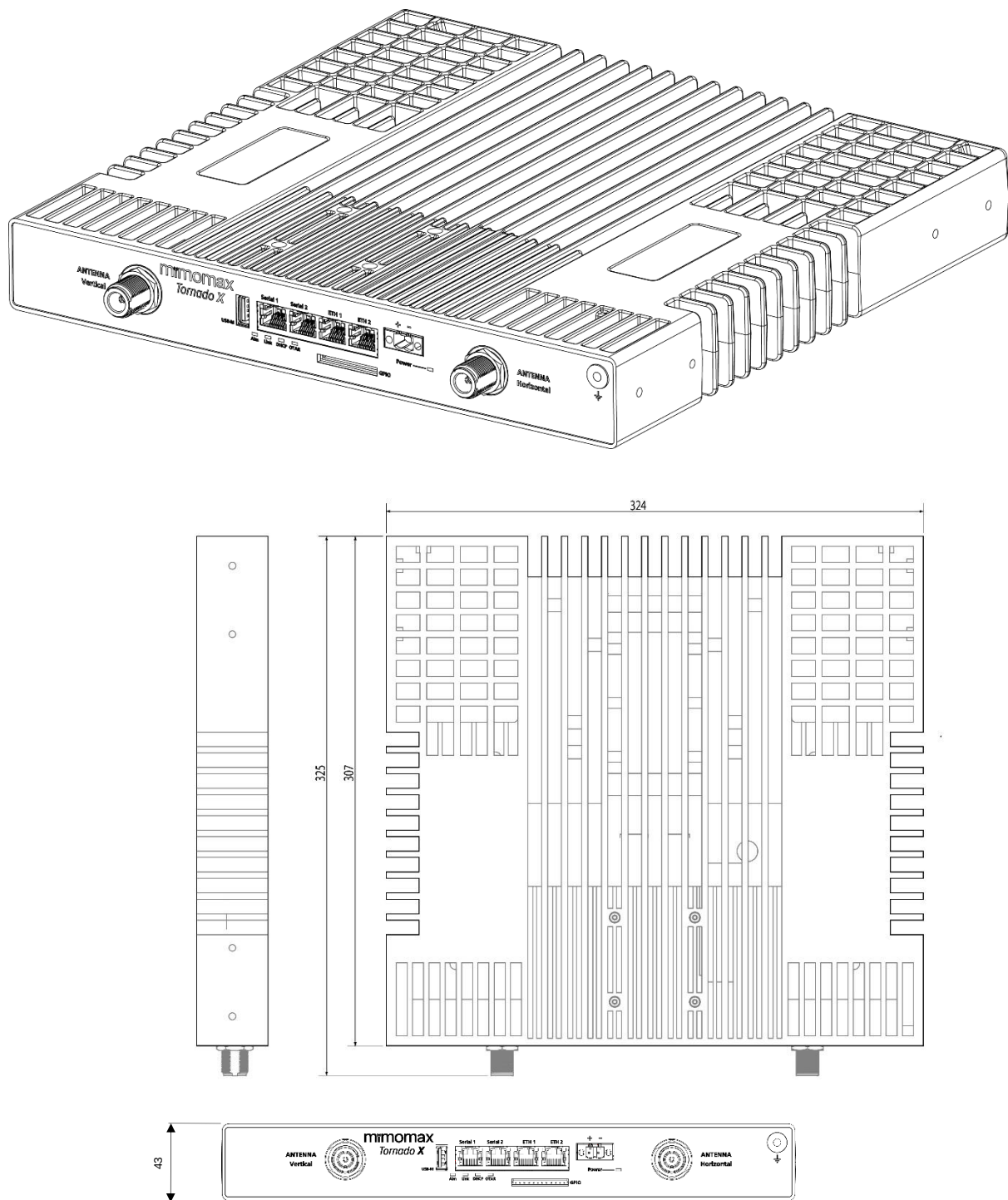
Mechanical Dimensions for Tornado X (All units are in mm)
