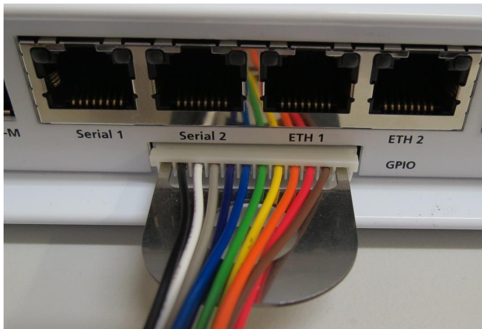
GPIO Connector
