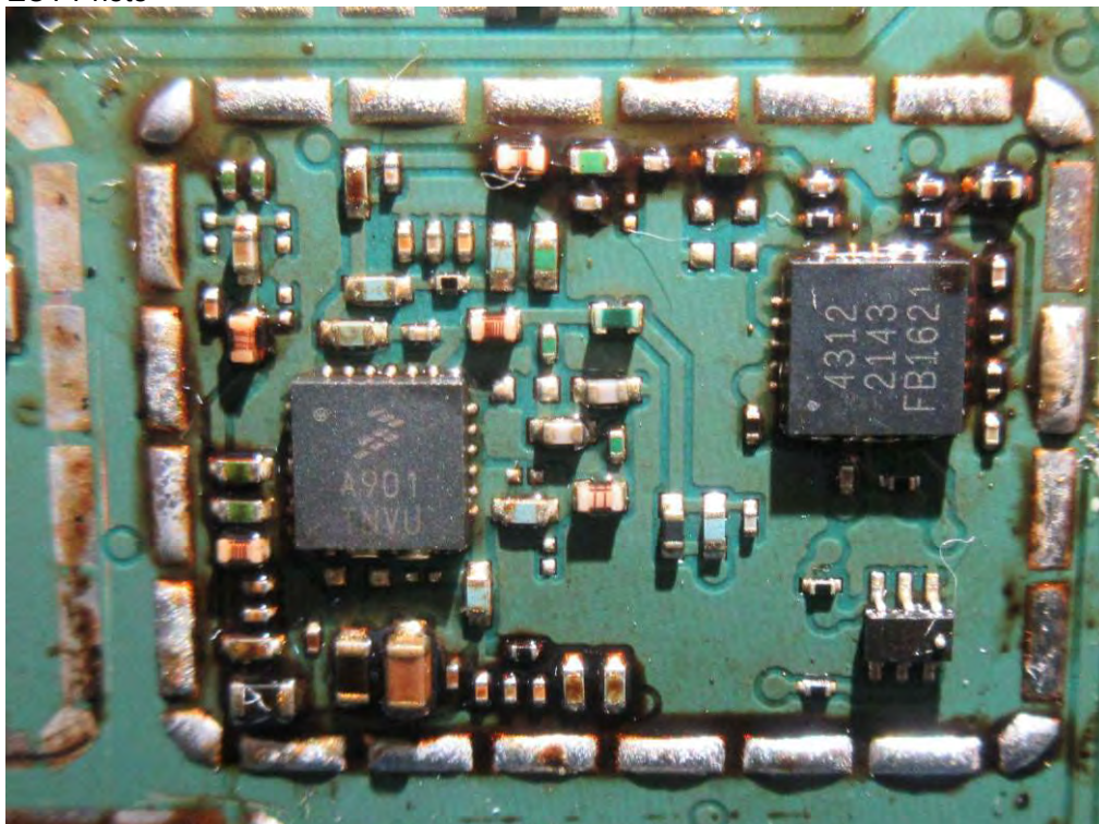
(76) EUT Photo
