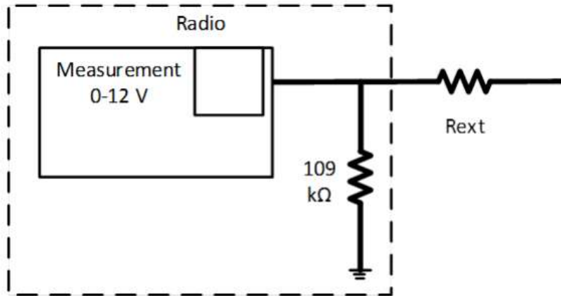
GPIO Input Circuit
