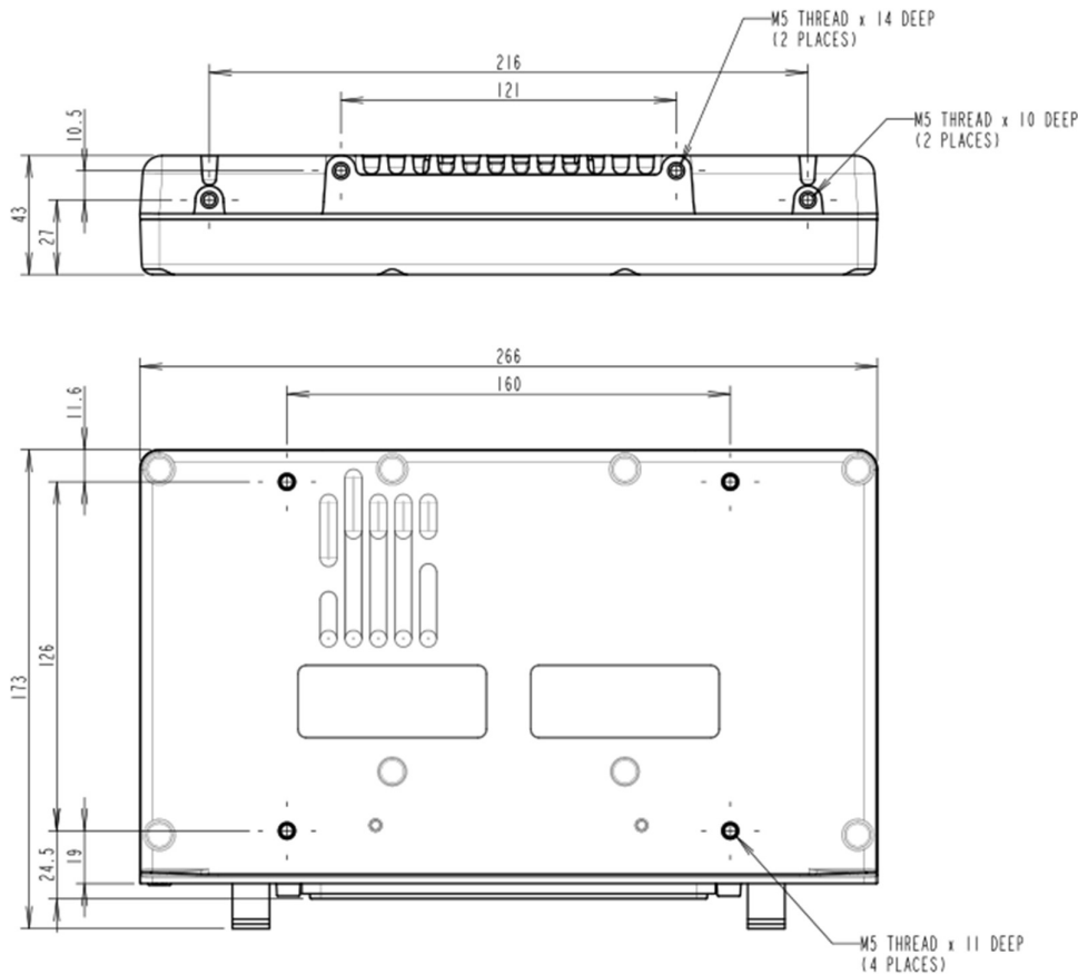
Mounting hole size, depth and location
