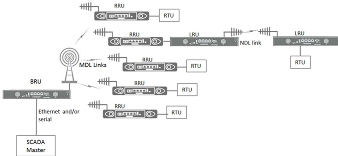
SCADA Network Example
