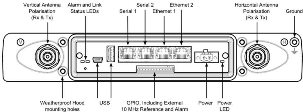
Tornado XR Connectors
