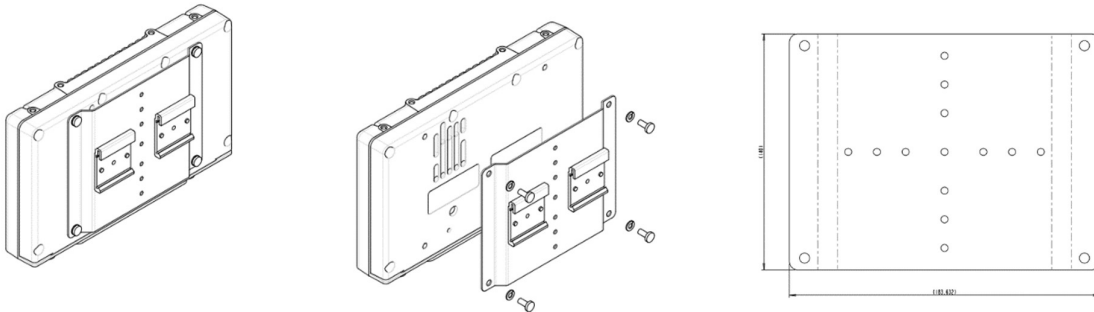
Tornado XR DIN mount dimension (in mm)
