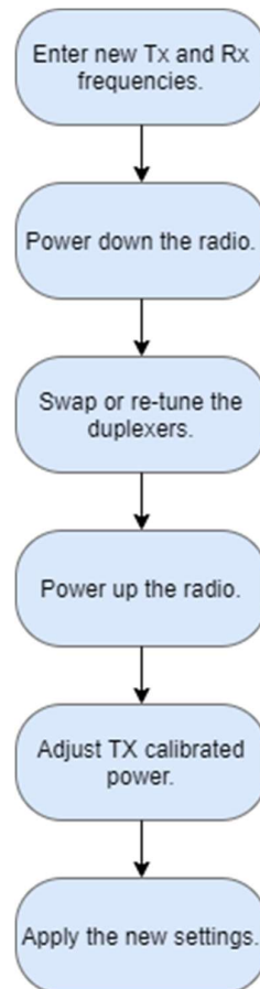
Frequency change process
