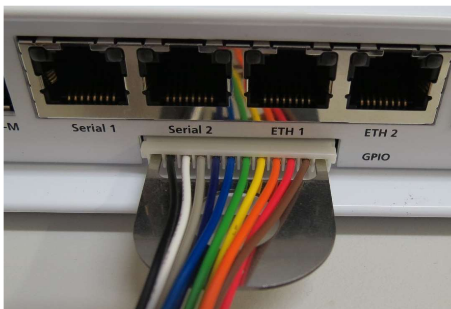
GPIO Connector
