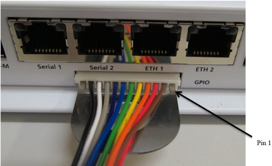
GPIO Connector
