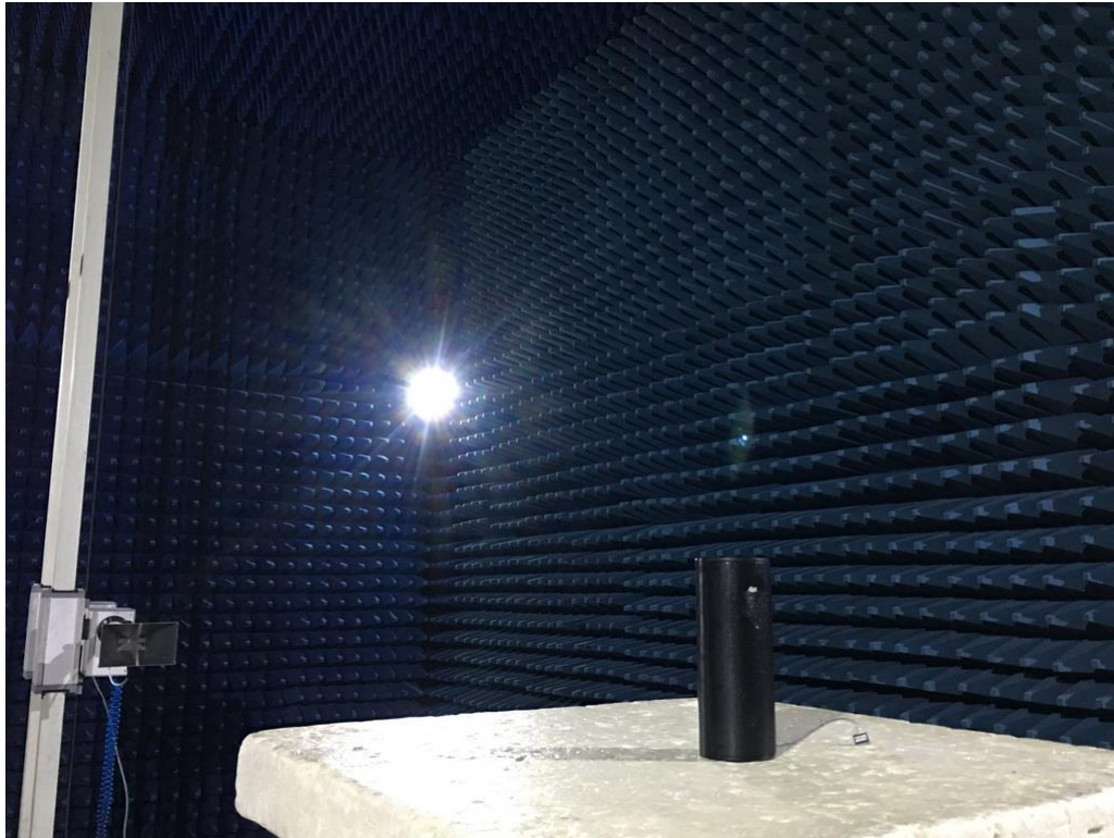
Photograph 3: Set-up for Spurious Emissions (1GHz-18GHz)
