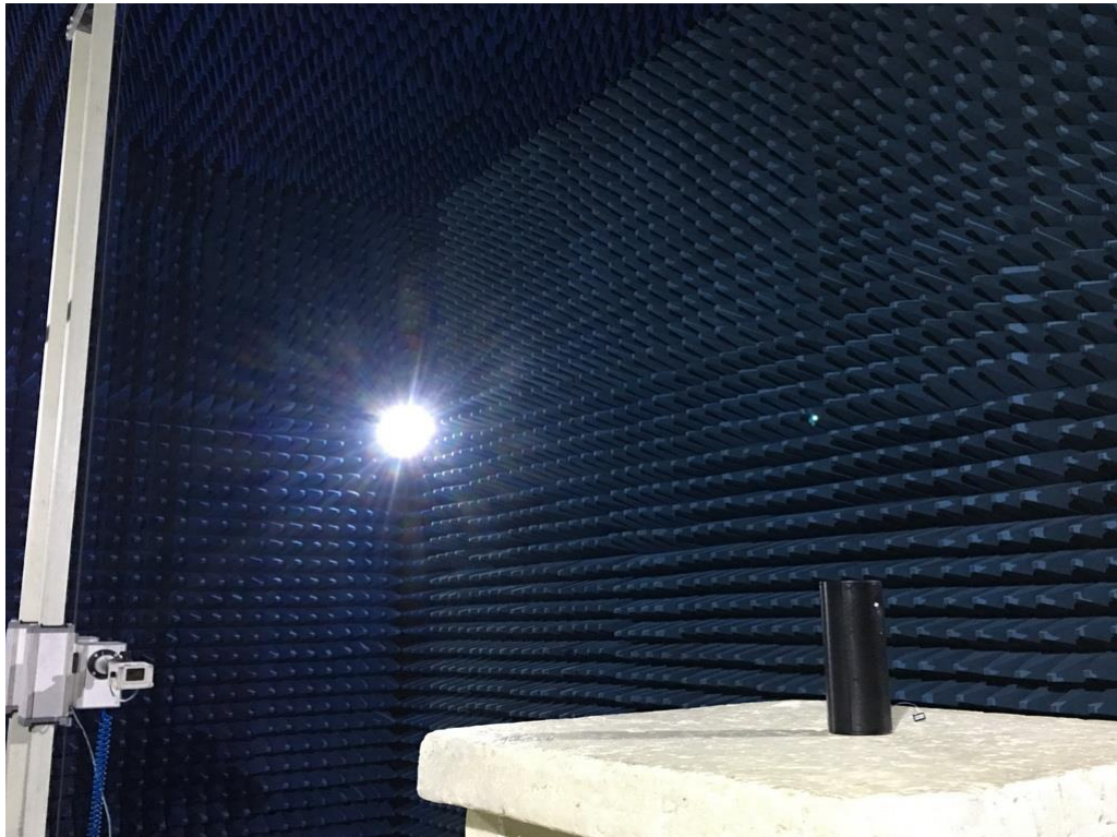
Photograph 4S: Set-up for Spurious Emissions (18GHz-26GHz)
