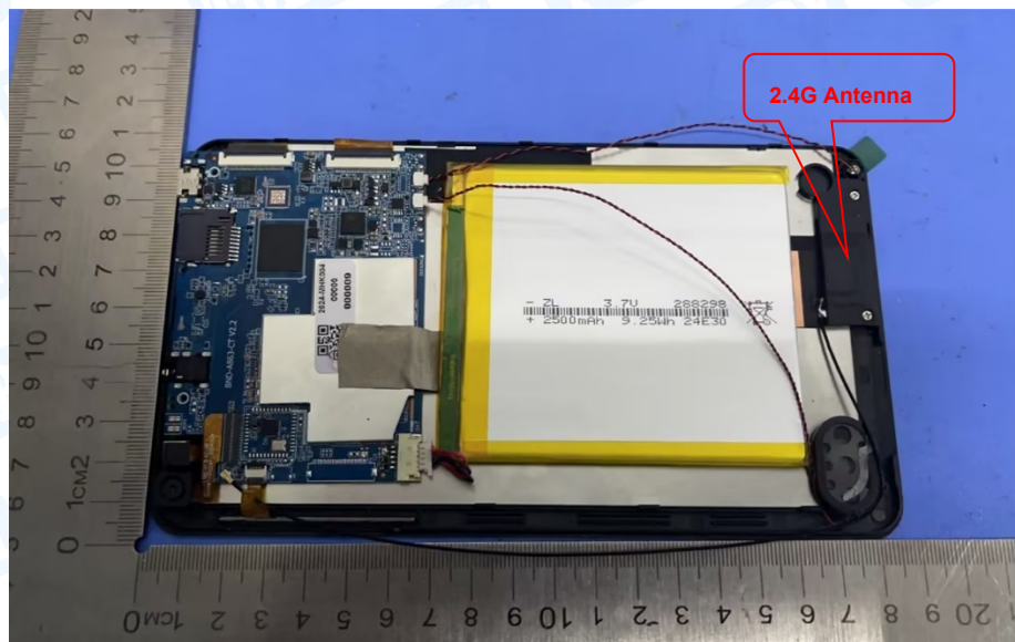
Photo 8 Internal of EUT
