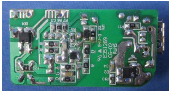
PCB side 2
