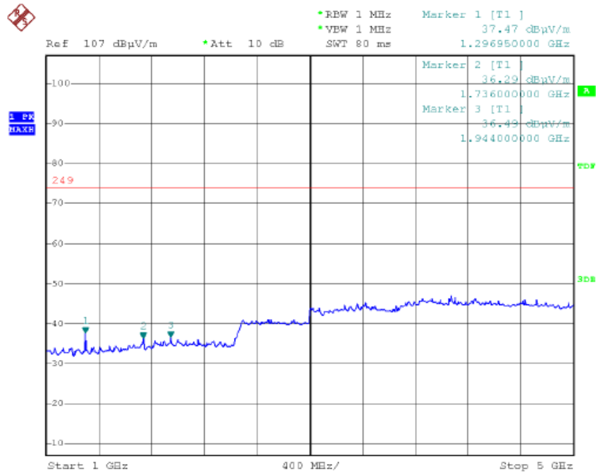
Test Plot of Above 1GHz(Horizontal Polarzation)
