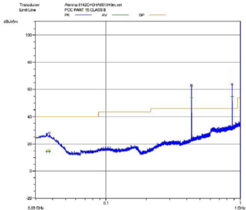
Test Plot of Below 1GHz(Vertical Polarzation)
