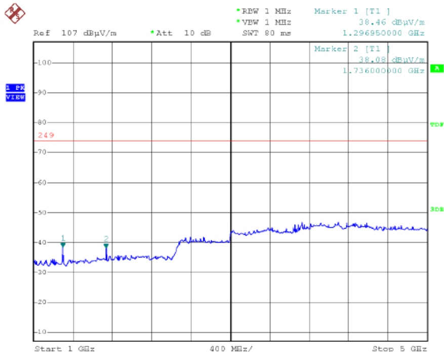
Test Plot of Above 1GHz(Vertical Polarzation)
