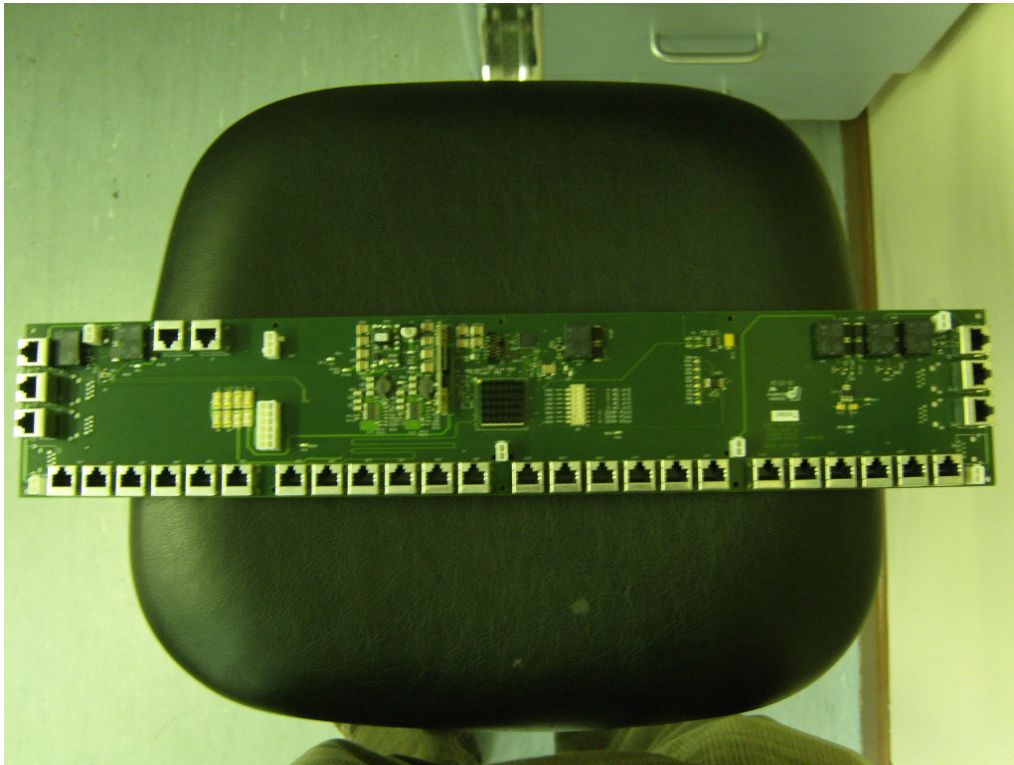
Photo 3: Internal - Trigger Board - Top
