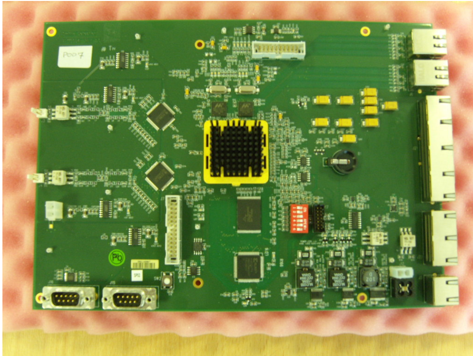
Photo 1: Internal - Digital Receiver Board – Top
