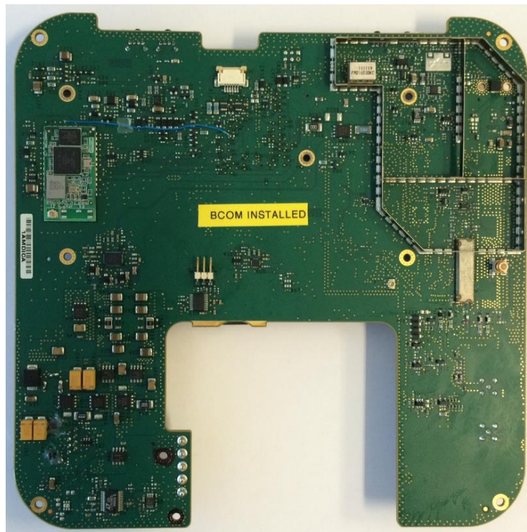
Interface board (out of housing), shield removed
