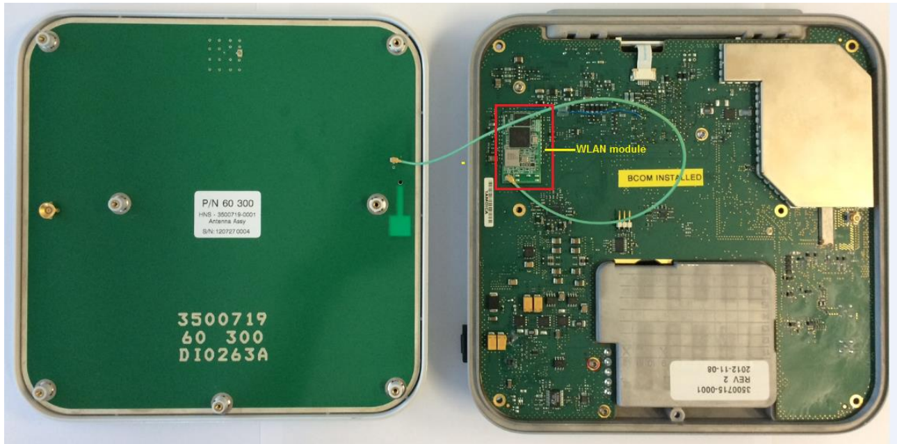
Back of radome
