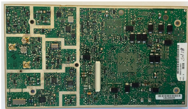
Satellite board (Underside)
