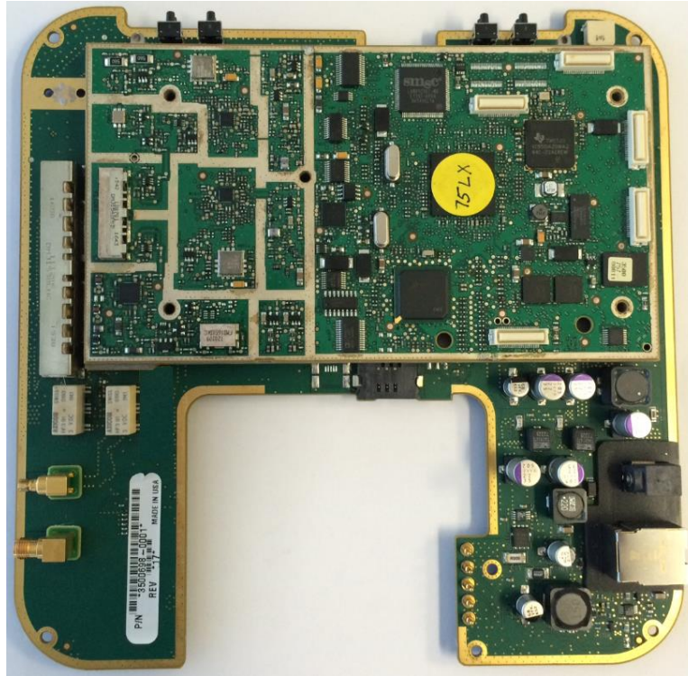
Interface board (underside) - with Satellite board (in housing) installed
