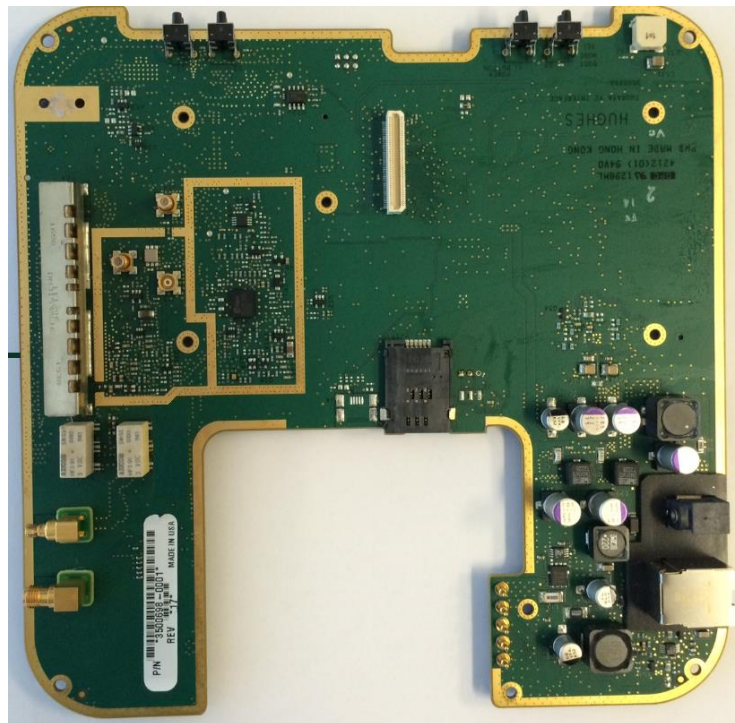
Interface board (underside) - with Satellite board and housing removed
