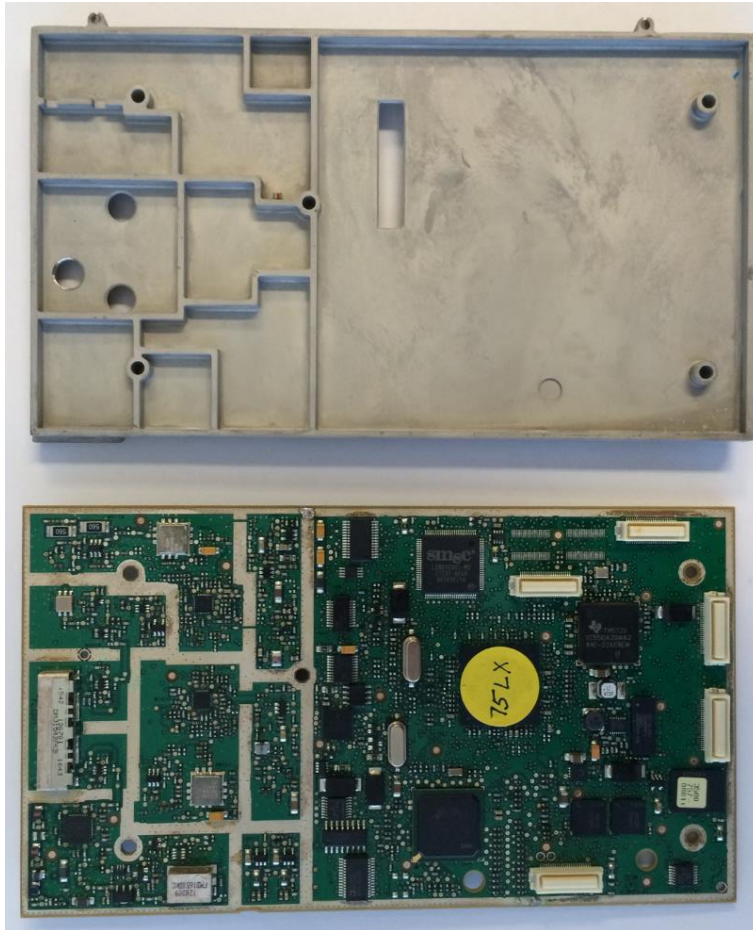
Satellite board (Topside) and housing
