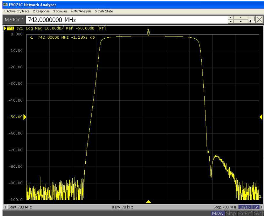
Down-link
