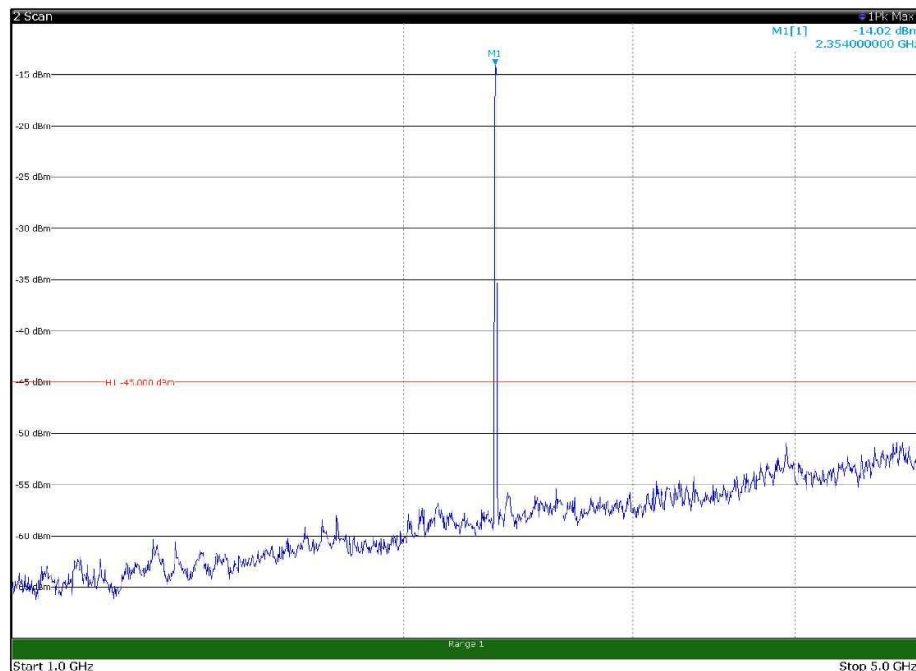
Channel: MIDDLE, Modulation: QPSK, BW=10MHz, Range: 1GHz - 5GHz, Polarization: Vertical
