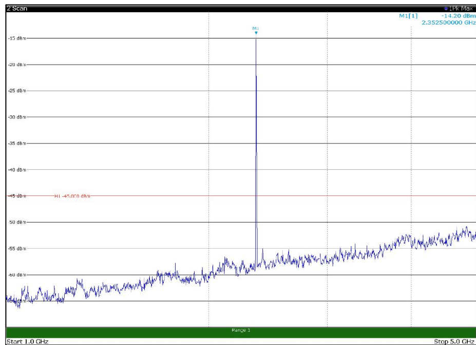
Channel: MIDDLE, Modulation: 256QAM, BW=5MHz, Range: 1GHz - 5GHz, Polarization: Vertical
