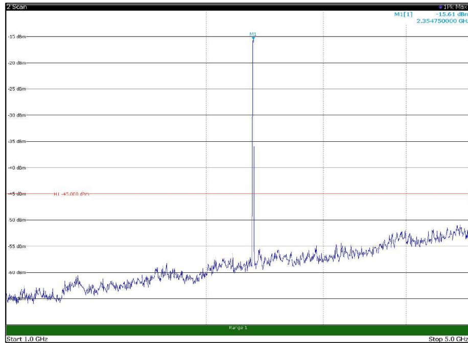
Channel: MIDDLE, Modulation: QPSK, BW=10MHz, Range: 1GHz - 5GHz, Polarization: Horizontal
