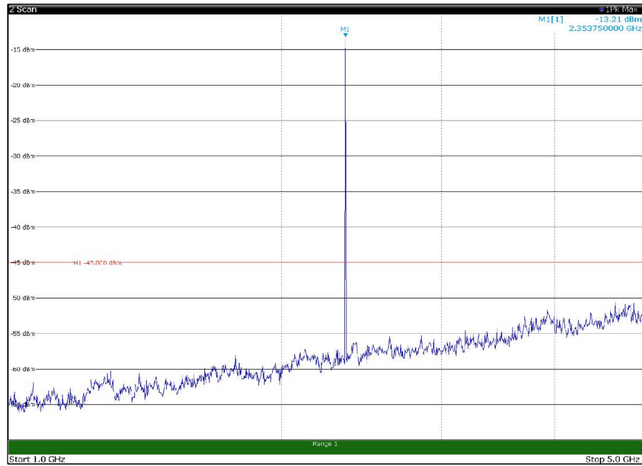
Channel: MIDDLE, Modulation: 256QAM, BW=5MHz, Range: 1GHz - 5GHz, Polarization: Horizontal
