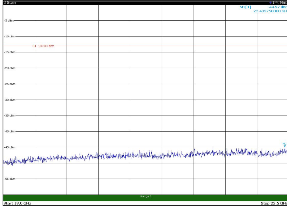
Channel: BOTTOM, Modulation: 16QAM, BW=5MHz, Range: 18GHz - 22.5GHz, Polarization: Vertical
