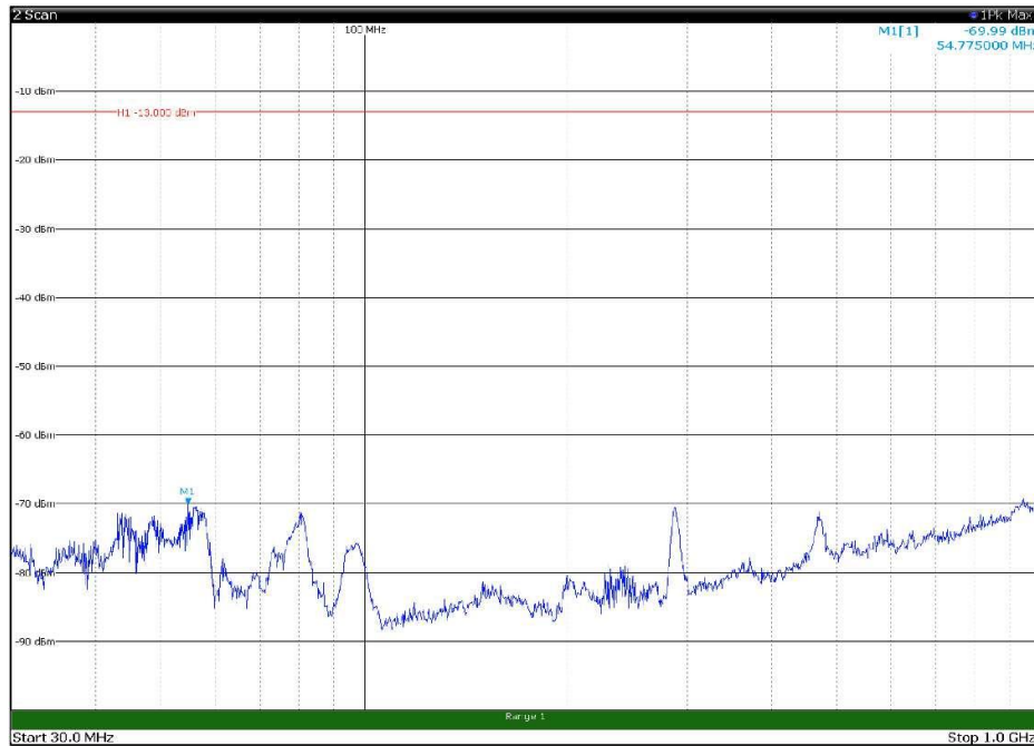
Channel: TOP, Modulation: 256QAM, BW=10MHz, Range: 30MHz - 1GHz, Polarization: Horizontal
