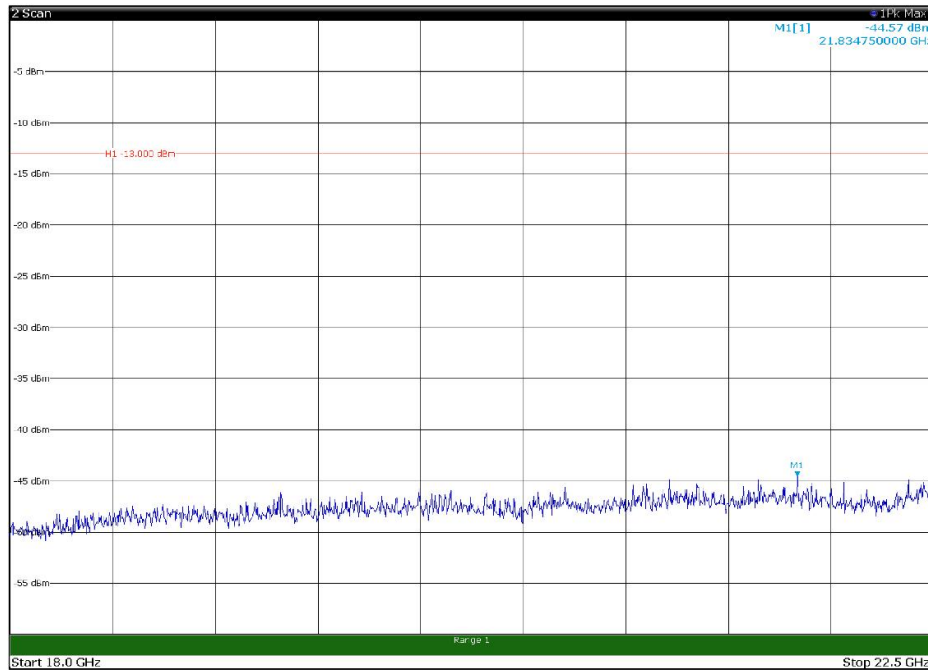
Channel: TOP, Modulation: 256QAM, BW=10MHz, Range: 18GHz - 22.5GHz, Polarization: Horizontal
