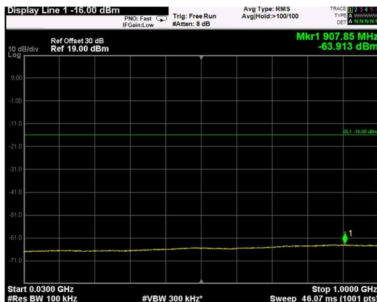
Channel: BOTTOM, Modulation: 256QAM, BW=20MHz, Range: Lower
