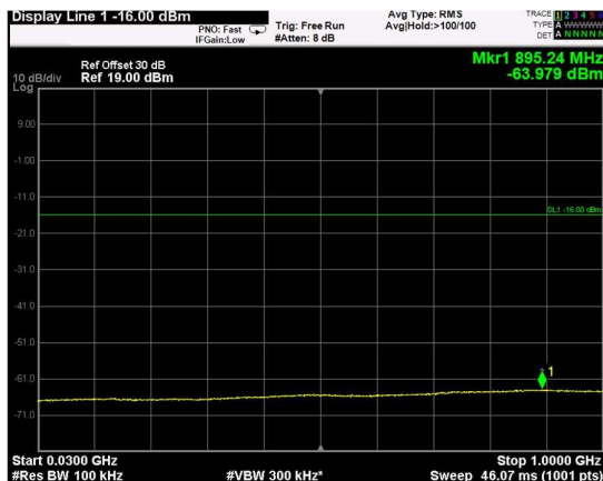
Channel: BOTTOM, Modulation: 16QAM, BW=20MHz, Range: Lower
