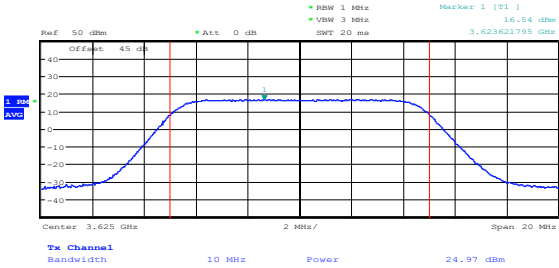
Figure 8.36-1: Output power and power density validation when maxEirp setting P_i = 29.7
