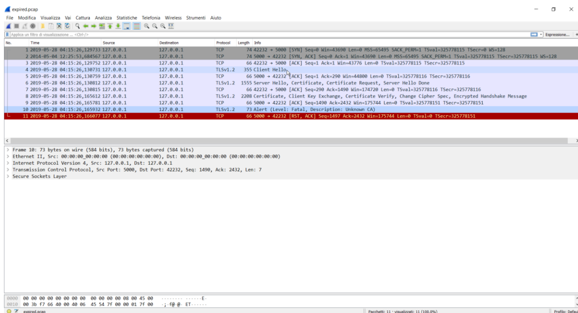
Figure 9.34-2: Alert Unknown CA
