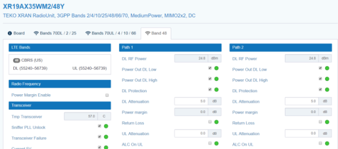
Figure 8.36-2: Setting of the power on GUI
