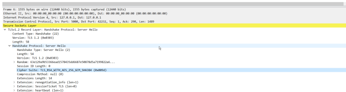
Figure 9.34-1: Client hello, Server hello
