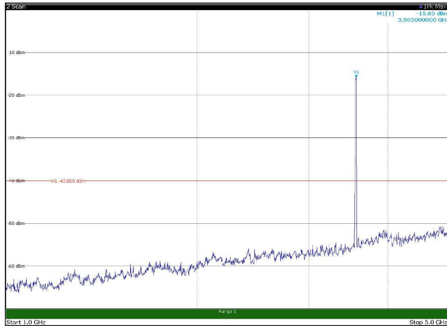
Channel: BOTTOM, Modulation: 16QAM, BW=20MHz, Range: 1GHz - 5GHz, Polarization: Horizontal
