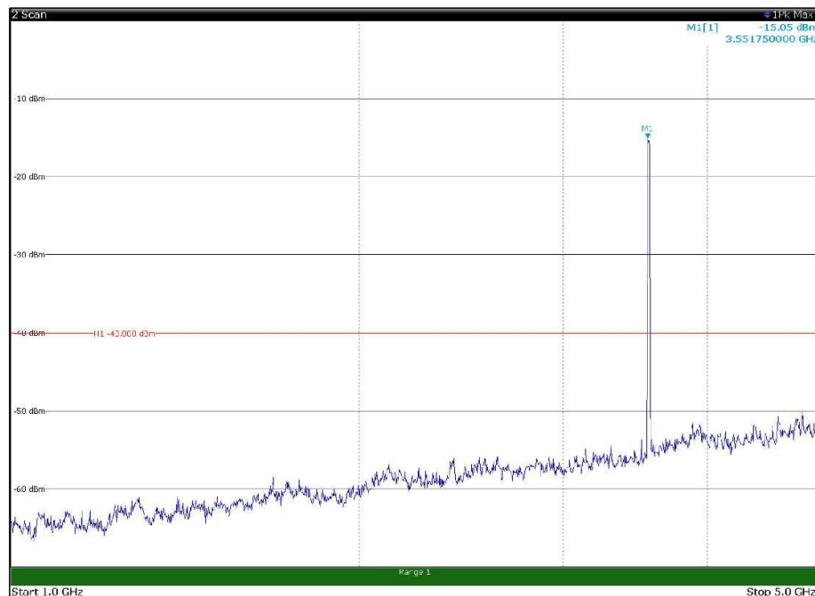
Channel: BOTTOM, Modulation: 16QAM, BW=20MHz, Range: 1GHz - 5GHz, Polarization: Vertical
