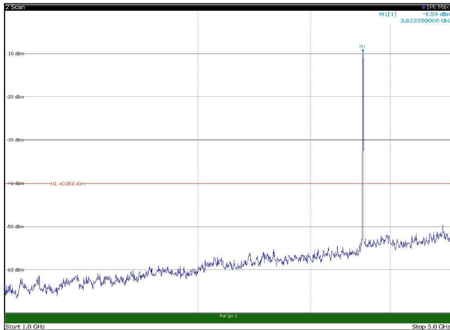
Channel: MIDDLE, Modulation: 16QAM, BW=15MHz, Range: 1GHz - 5GHz, Polarization: Vertical
