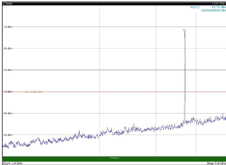
Channel: TOP, Modulation: QPSK, BW=15MHz, Range: 1GHz - 5GHz, Polarization: Vertical
