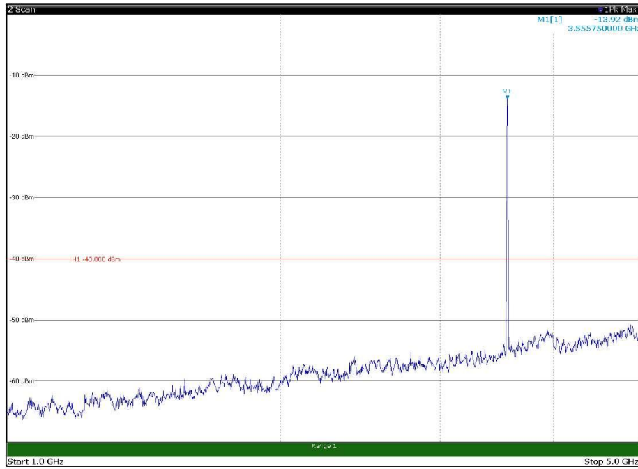
Channel: BOTTOM, Modulation: 16QAM, BW=15MHz, Range: 1GHz - 5GHz, Polarization: Horizontal
