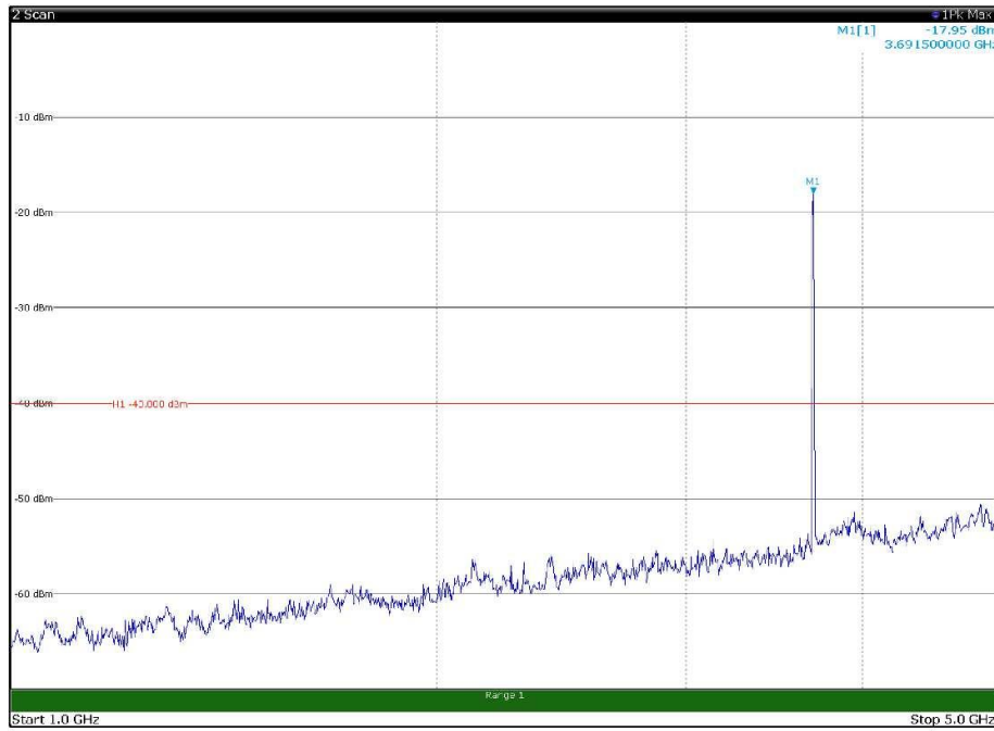
Channel: TOP, Modulation: QPSK, BW=15MHz, Range: 1GHz - 5GHz, Polarization: Horizontal
