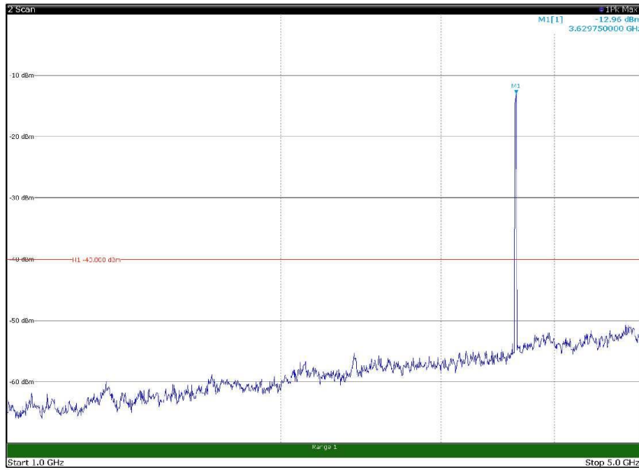
Channel: MIDDLE, Modulation: 16QAM, BW=15MHz, Range: 1GHz - 5GHz, Polarization: Horizontal
