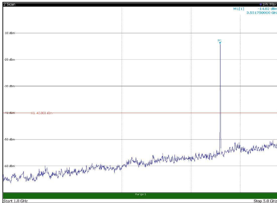
Channel: BOTTOM, Modulation: 16QAM, BW=15MHz, Range: 1GHz - 5GHz, Polarization: Vertical
