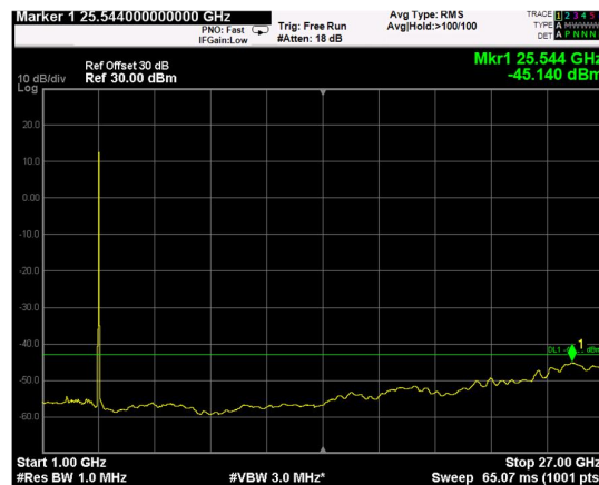
Channel: TOP, Modulation: 16QAM, BW=15MHz, Range: 1GHz - 27GHz
