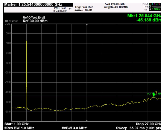
Channel: MIDDLE, Modulation: 16QAM, BW=10MHz, Range: 1GHz - 27GHz
