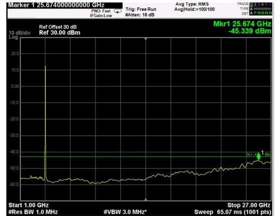
Channel: BOTTOM, Modulation: 64QAM, BW=10MHz, Range: 1GHz - 27GHz
