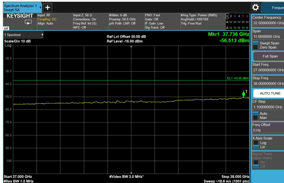
Channel: TOP, Modulation: 16QAM, BW=10MHz, Range: 27GHz - 38GHz
