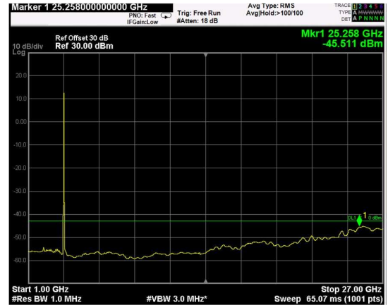
Channel: MIDDLE, Modulation: 16QAM, BW=10MHz, Range: 1GHz - 27GHz
