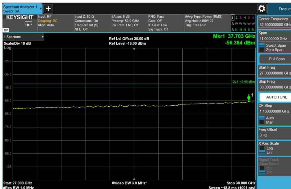
Channel: TOP, Modulation: 256QAM, BW=5, Range: 27GHz - 38GHz
