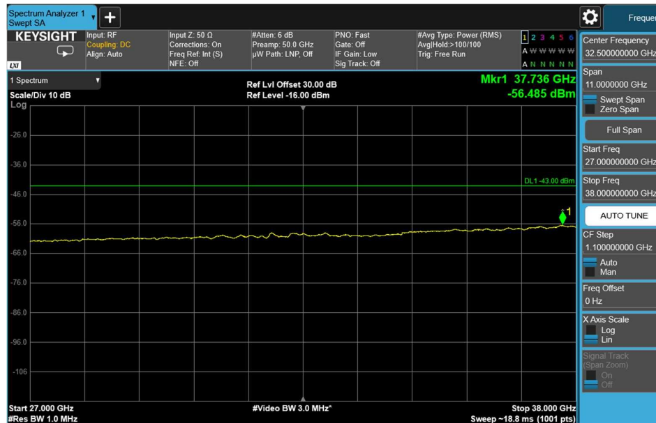
Channel: MIDDLE, Modulation: 64QAM, BW=10MHz, Range: 27GHz - 38GHz
