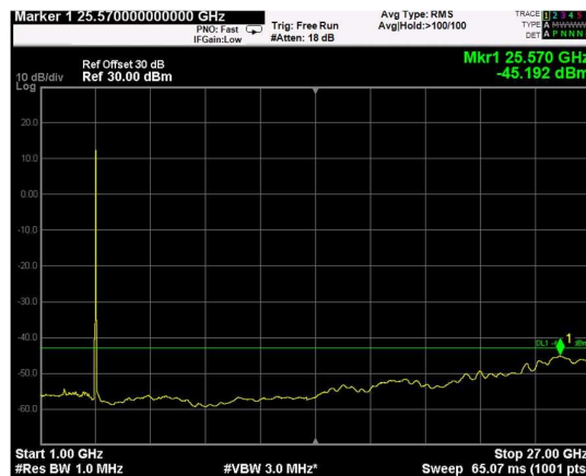
Channel: MIDDLE, Modulation: QPSK, BW=10MHz, Range: 1GHz - 27GHz
