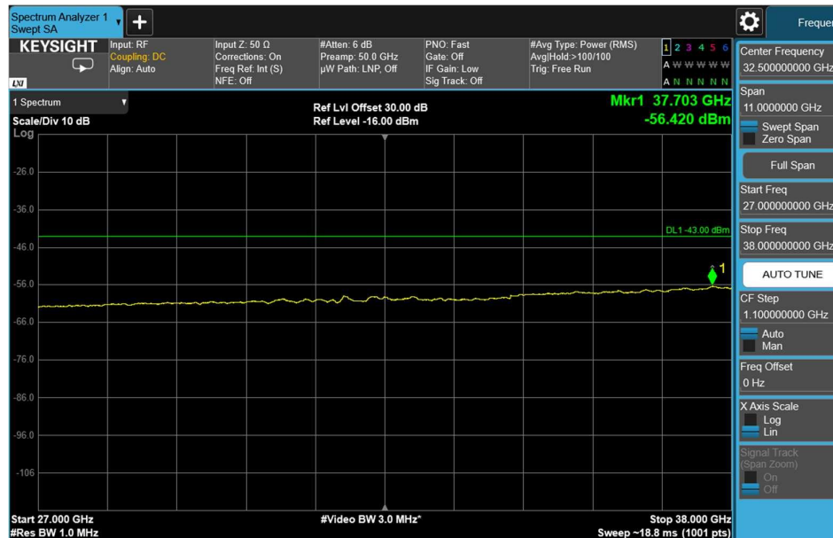
Channel: TOP, Modulation: QPSK, BW=10MHz, Range: 27GHz - 38GHz
