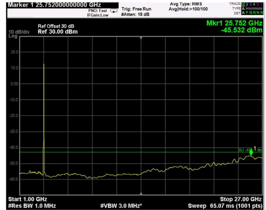
Channel: TOP, Modulation: 16QAM, BW=10MHz, Range: 1GHz - 27GHz
