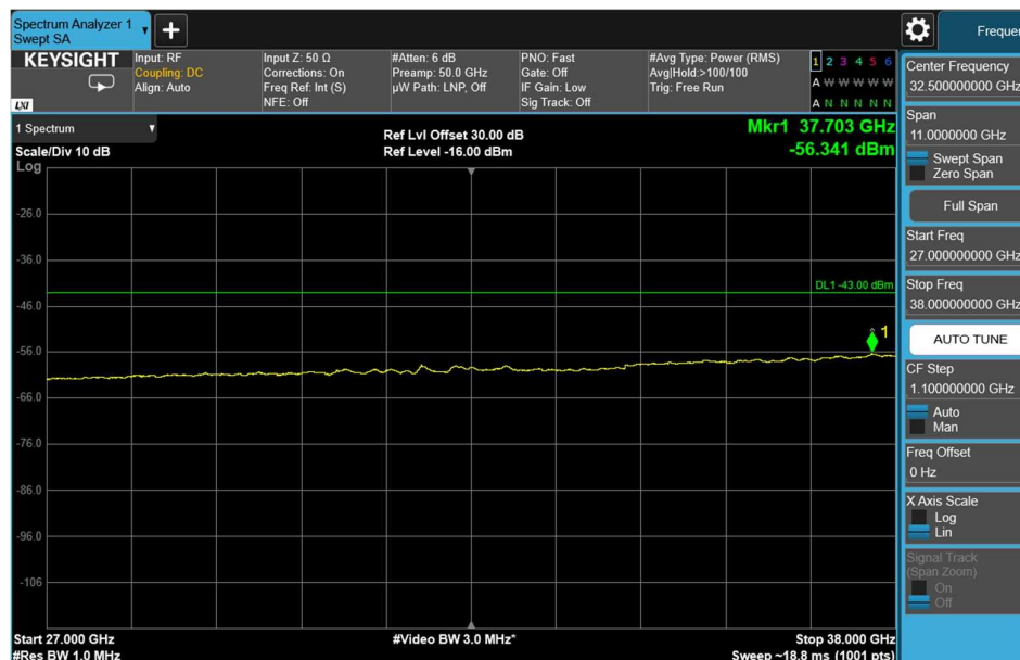
Channel: TOP, Modulation: QPSK, BW=5MHz, Range: 27GHz - 38GHz
