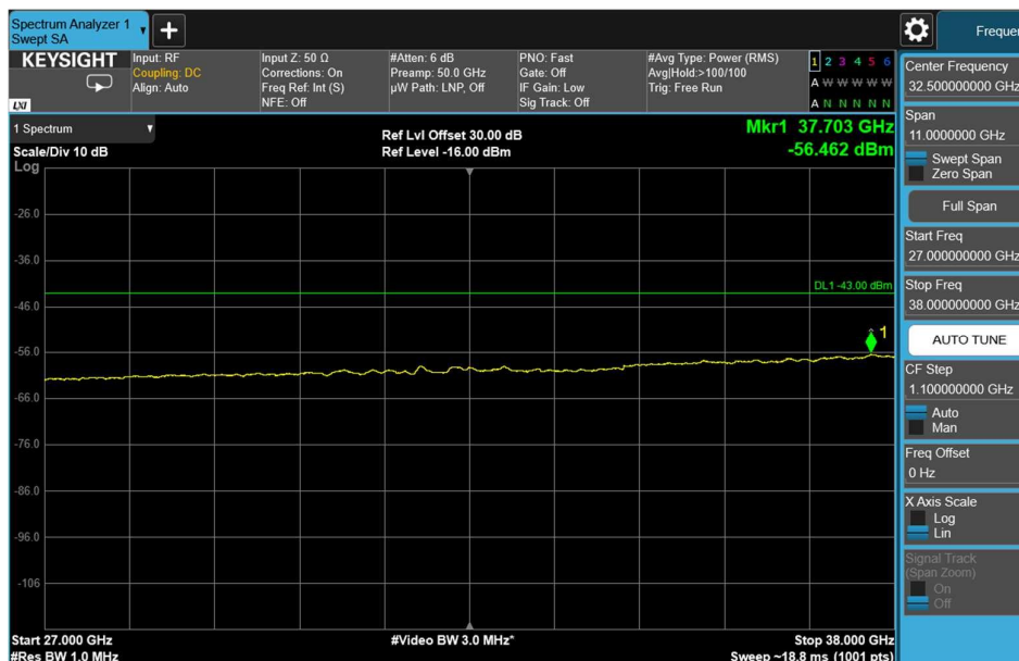
Channel: MIDDLE, Modulation: QPSK, BW=10MHz, Range: 27GHz - 38GHz
