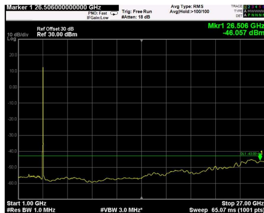
Channel: BOTTOM, Modulation: 64QAM, BW=5MHz, Range: 1GHz - 27GHz
