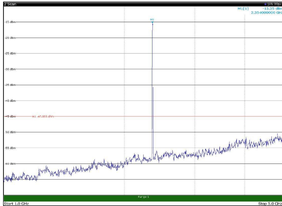
Channel: MIDDLE, Modulation: 256QAM, BW=10MHz, Range: 1GHz - 5GHz, Polarization: Horizontal
