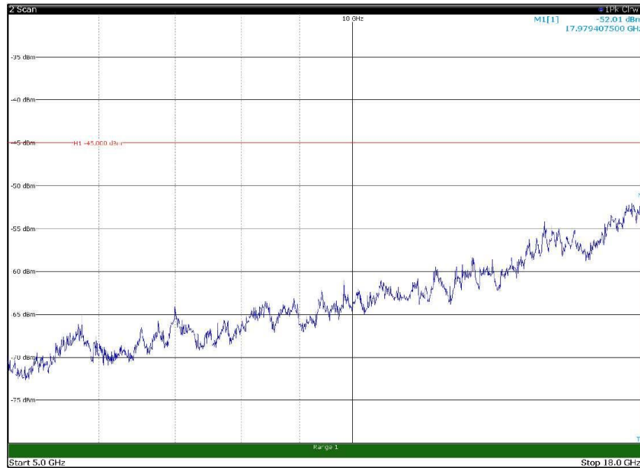
Channel: MIDDLE, Modulation: 16QAM, BW=10MHz, Range: 5GHz - 18GHz, Polarization: Horizontal
