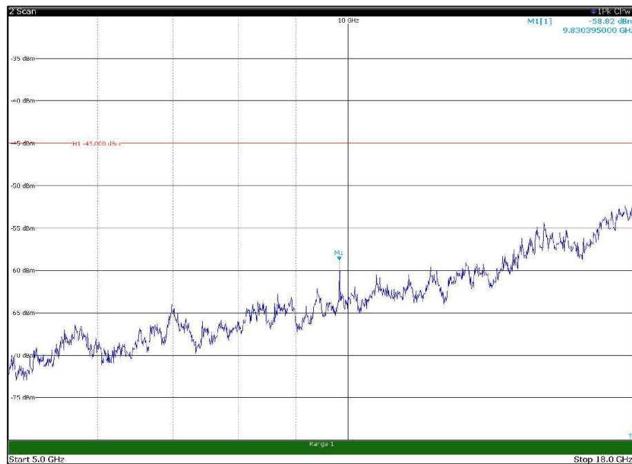
Channel: MIDDLE, Modulation: 16QAM, BW=10MHz, Range: 5GHz - 18GHz, Polarization: Vertical
