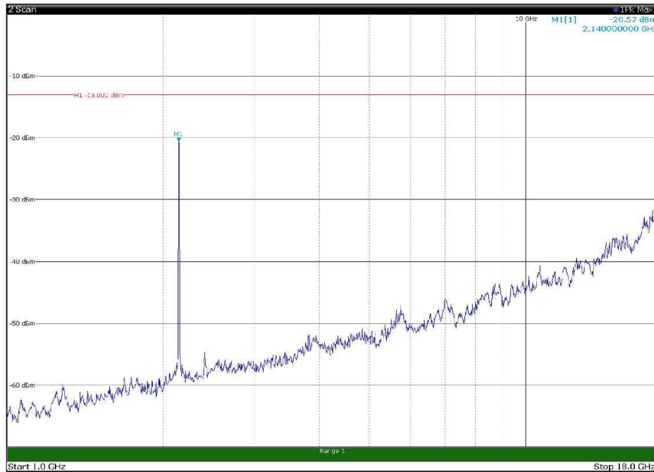
Channel: MIDDLE, Modulation: 16QAM, BW=15MHz, Range: 1GHz - 18GHz, Polarization: Horizontal
