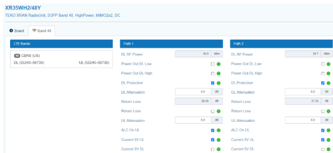
Figure 7.55-1: Output power and power density validation when maxEirp setting P_i = 37
