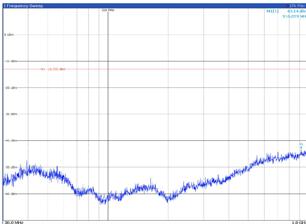
Channel: MIDDLE, Modulation: 64QAM, BW=50MHz, Range: 30MHz - 1GHz, Polarization: Horizontal
