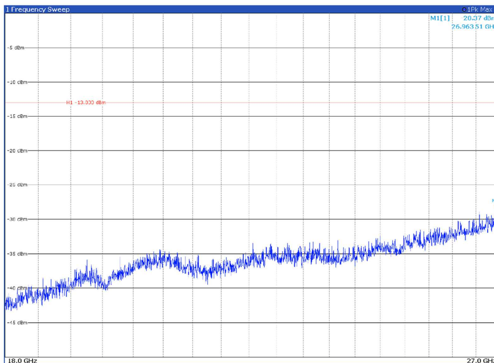
Channel: MIDDLE, Modulation: 64QAM, BW=20MHz, Range: 18GHz - 27GHz, Polarization: Horizontal
