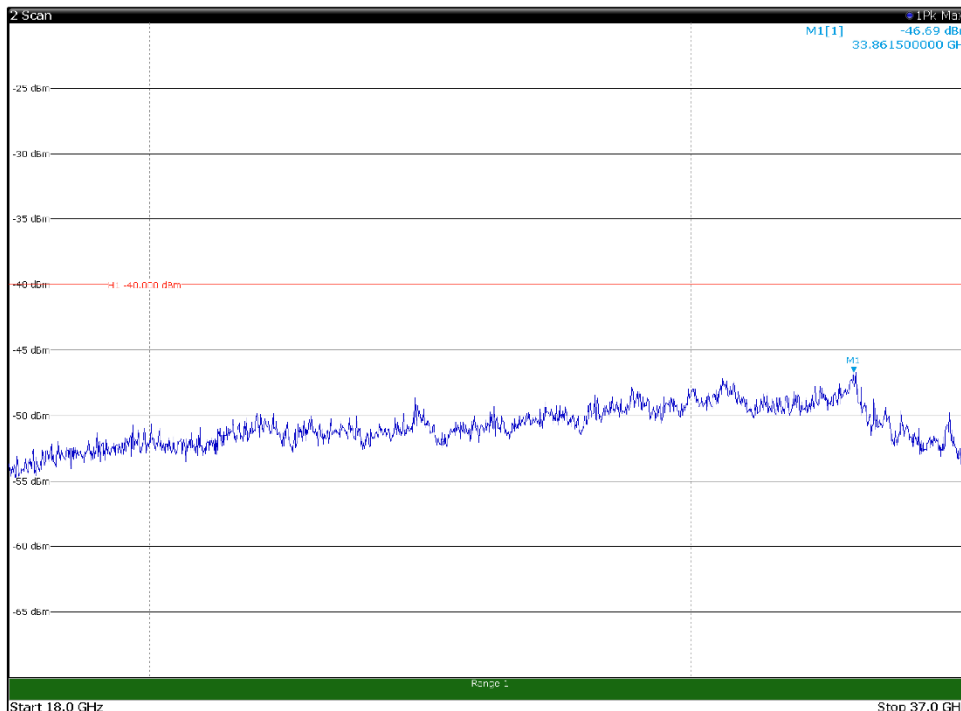
Channel: TOP, Modulation: 16QAM, BW=20MHz, Range: 18GHz - 37GHz, Polarization: Vertical
