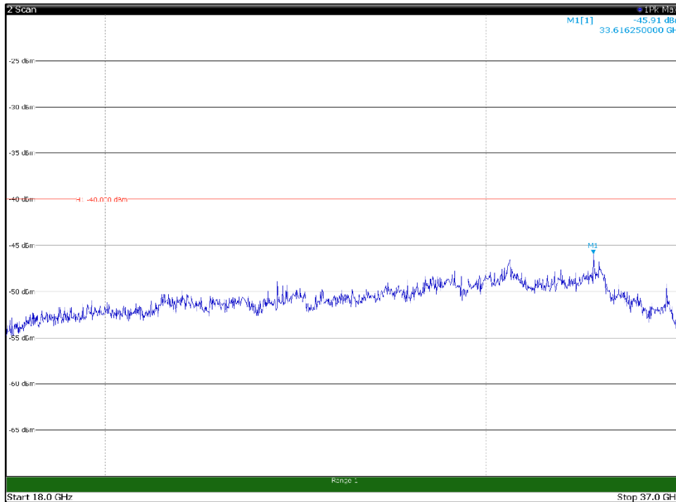
Channel: TOP, Modulation: 16QAM, BW=20MHz, Range: 18GHz - 37GHz, Polarization: Horizontal
