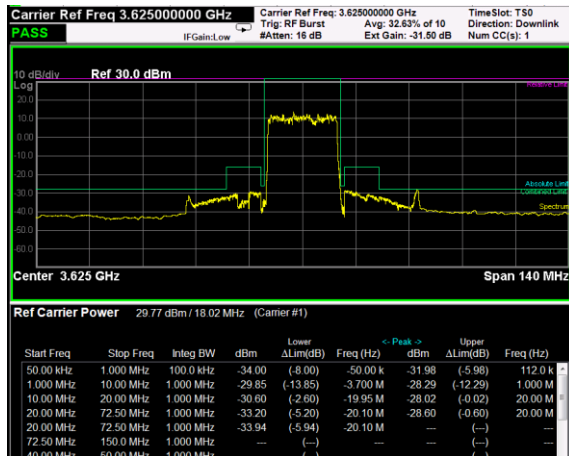
Middle Band Edge, 1 Carrier, Modulation: 64QAM, BW=20MHz
