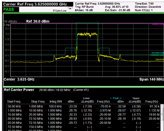
Middle Band Edge, 1 Carrier, Modulation: 16QAM, BW=20MHz
