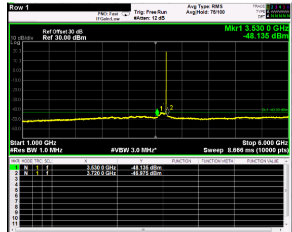
Channel: TOP, Modulation: 16QAM, BW=5MHz, Range: 1GHz - 6GHz
