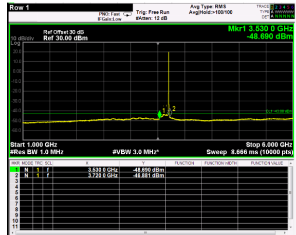
Channel: TOP, Modulation: QPSK, BW=5MHz, Range: 1GHz - 6GHz
