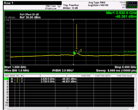
Channel: MIDDLE, Modulation: 256QAM, BW=10MHz, Range: 1GHz - 6GHz
