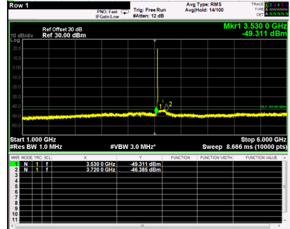
Channel: BOTTOM, Modulation: QPSK, BW=5MHz, Range: 1GHz - 6GHz
