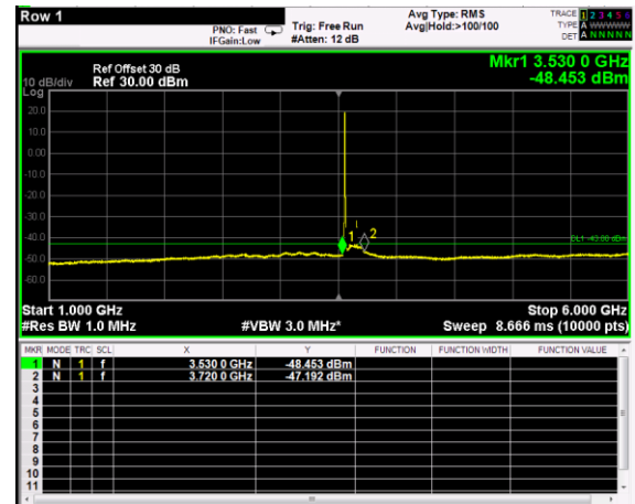
Channel: BOTTOM, Modulation: 256QAM, BW=5MHz, Range: 1GHz - 6GHz
