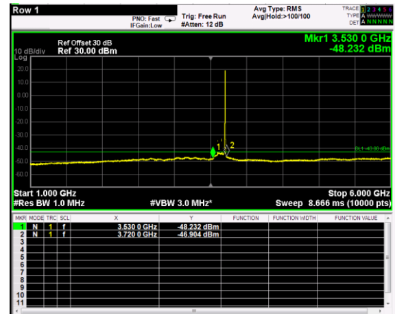
Channel: TOP, Modulation: 64QAM, BW=5MHz, Range: 1GHz - 6GHz
