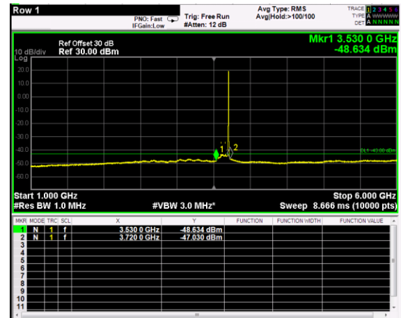
Channel: TOP, Modulation: 256QAM, BW=5MHz, Range: 1GHz - 6GHz
