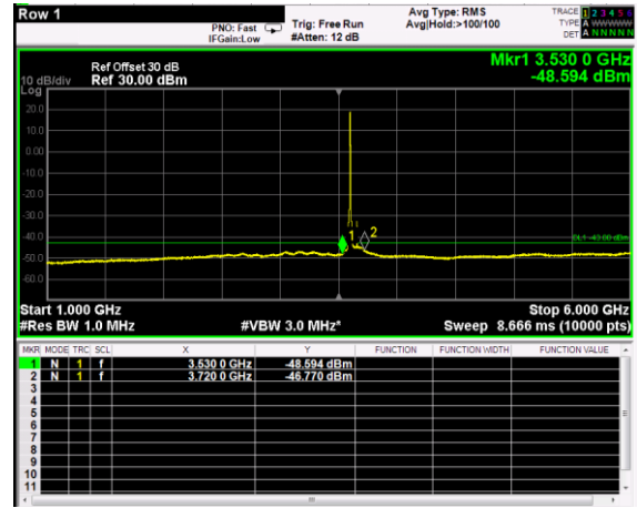
Channel: BOTTOM, Modulation: 16QAM, BW=10MHz, Range: 1GHz - 6GHz
