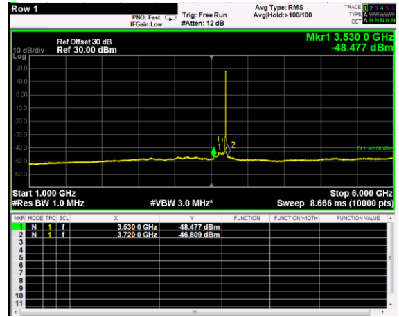
Channel: TOP, Modulation: 64QAM, BW=10MHz, Range: 1GHz - 6GHz
