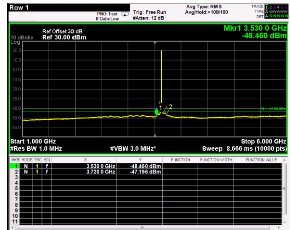
Channel: MIDDLE, Modulation: 16QAM, BW=5MHz, Range: 1GHz - 6GHz
