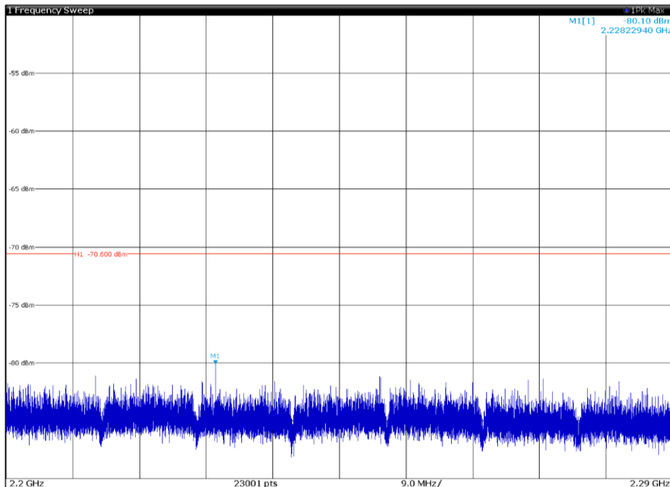
Channel: TOP, Modulation: 64QAM, BW=5MHz, Range: 2200MHz-2290GHz, Polarization: Vertical
