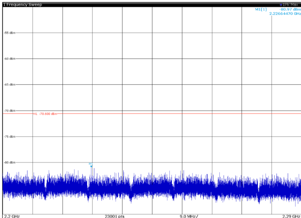
Channel: MIDDLE, Modulation: 256QAM, BW=10MHz, Range: 2200MHz-2290GHz, Polarization: Vertical
