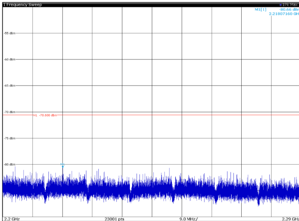
Channel: MIDDLE, Modulation: QPSK, BW=15MHz, Range: 2200MHz-2290GHz, Polarization: Vertical
