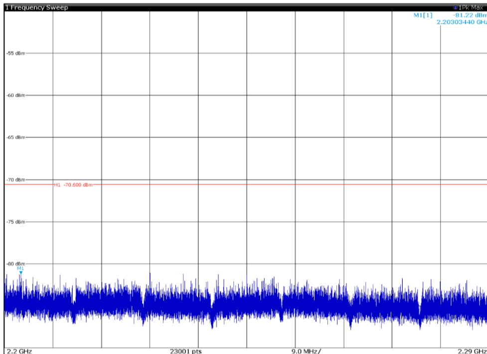
Channel: TOP, Modulation: 256QAM, BW=5MHz, Range: 2200MHz-2290GHz, Polarization: Vertical
