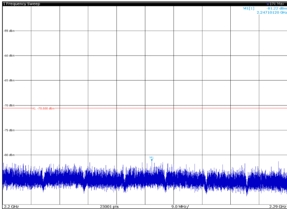
Channel: MIDDLE, Modulation: 256QAM, BW=10MHz, Range: 2200MHz-2290GHz, Polarization: Horizontal
