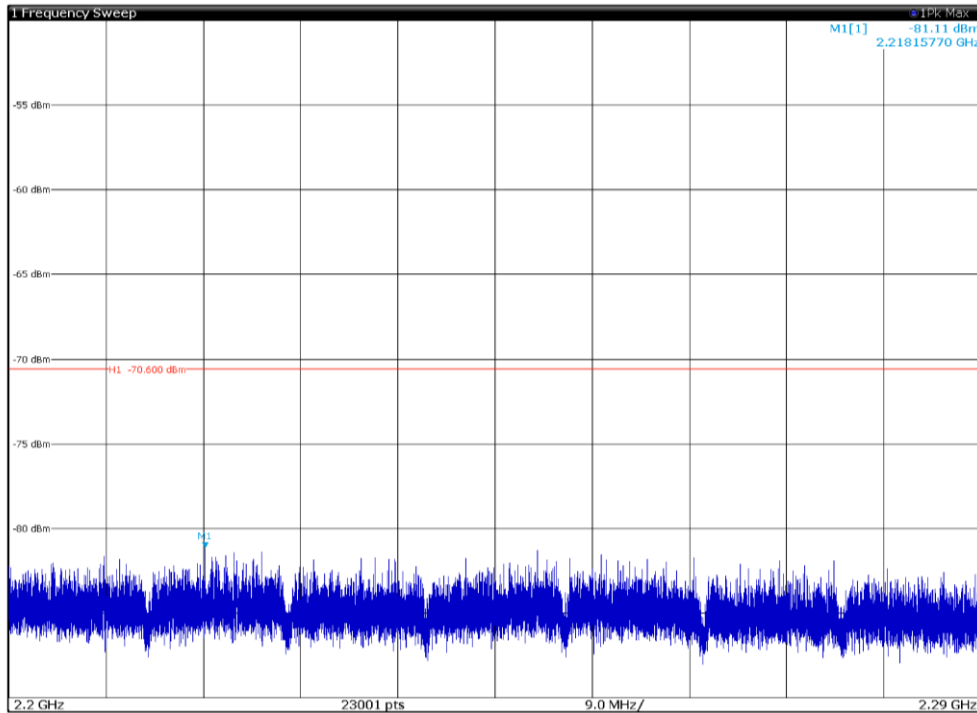
Channel: TOP, Modulation: 64QAM, BW=5MHz, Range: 2200MHz-2290GHz, Polarization: Horizontal
