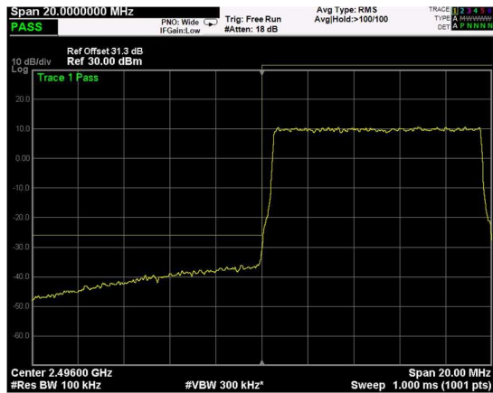
Low Band Edge, 1 Carrier, Modulation: 256QAM, BW=10MHz
