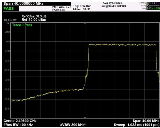
Low Band Edge, 1 Carrier, Modulation: QPSK, BW=20MHz
