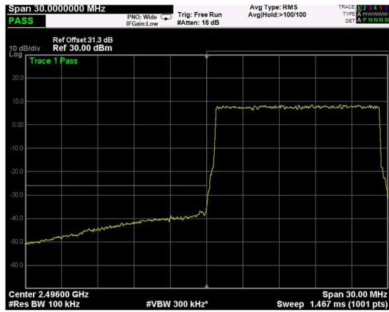
Low Band Edge, 1 Carrier, Modulation: QPSK, BW=15MHz
