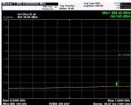
Channel: TOP, Modulation: 256QAM, BW=20MHz, Range: Lower
