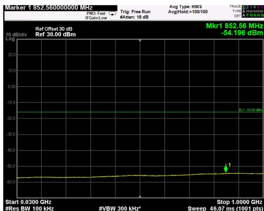
Channel: TOP, Modulation: 16QAM, BW=20MHz, Range: Lower
