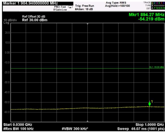
Channel: BOTTOM, Modulation: 16QAM, BW=15MHz, Range: Lower
