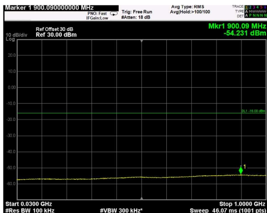
Channel: TOP, Modulation: 256QAM, BW=15MHz, Range: Lower
