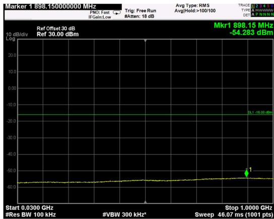
Channel: BOTTOM, Modulation: 256QAM, BW=5MHz, Range: Lower
