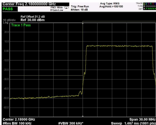
Low Band Edge, 1 Carrier, Modulation: 16QAM, BW=15MHz
