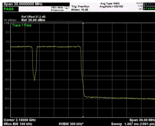
High Band Edge, 2 Carrier, Modulation: QPSK, BW=10MHz
