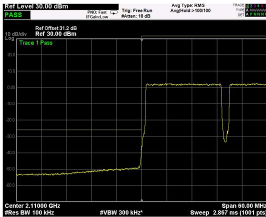
Low Band Edge, 2 Carrier, Modulation: 256QAM, BW=20MHz
