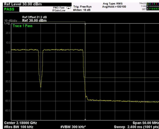
High Band Edge, 2 Carrier, Modulation: QPSK, BW=15MHz
