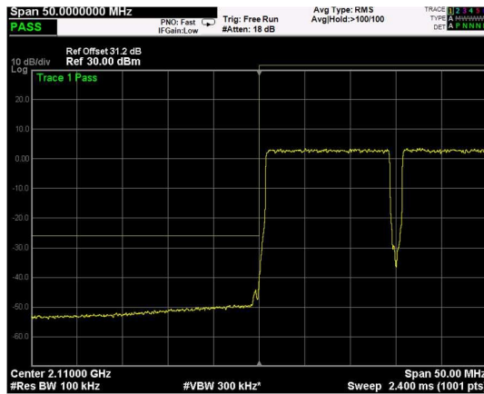
Low Band Edge, 2 Carrier, Modulation: 256QAM, BW=15MHz
