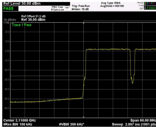
Low Band Edge, 2 Carrier, Modulation: QPSK, BW=20MHz
