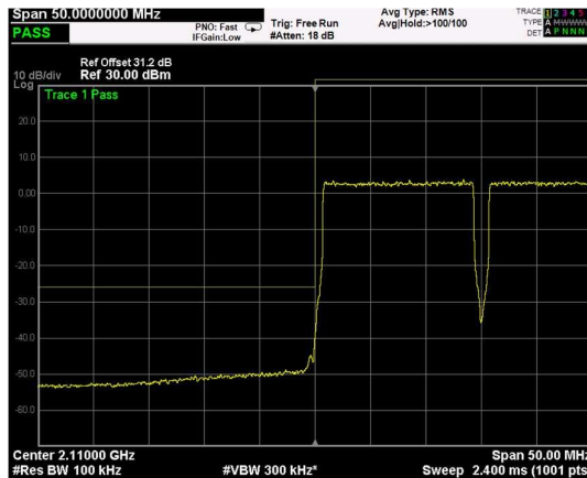
Low Band Edge, 2 Carrier, Modulation: 16QAM, BW=15MHz
