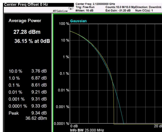
Channel: BOTTOM, Modulation: 16QAM, BW=20MHz, CCDF
