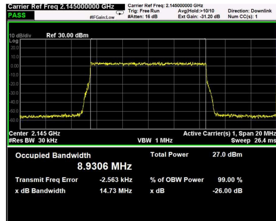
Channel: MIDDLE, Modulation: 16QAM, BW=10MHz
