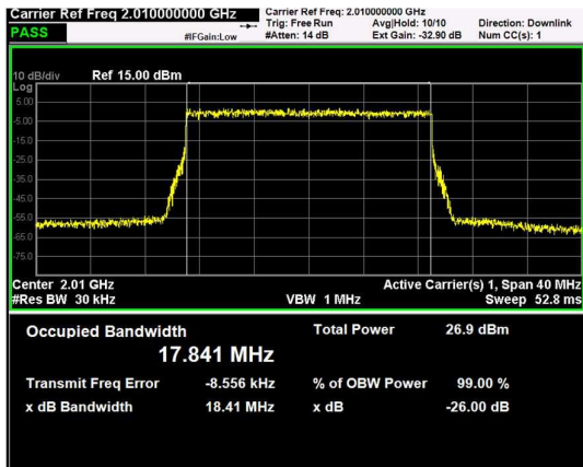
Channel: TOP, Modulation: 64QAM, BW=20MHz
