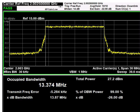
Channel: BOTTOM, Modulation: 16QAM, BW=15MHz
