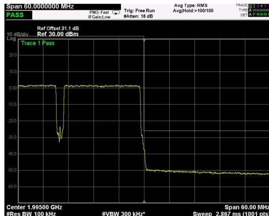
High Band Edge, 2 Carrier, Modulation: 64QAM, BW=20MHz
