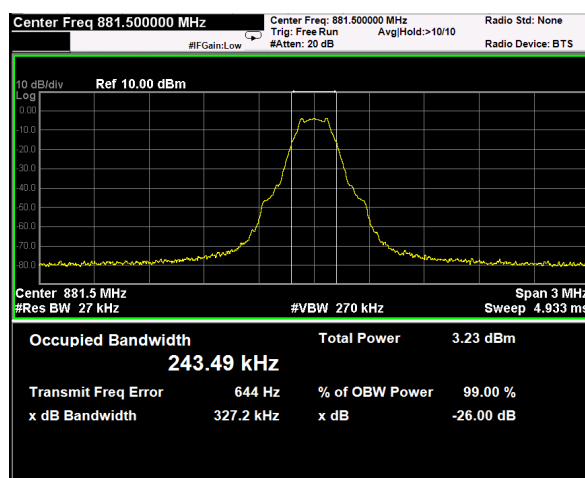
MSK Signal, Nominal Input Signal +3dB, Input
