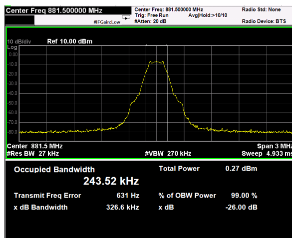
MSK Signal, Nominal Input Signal, Input
