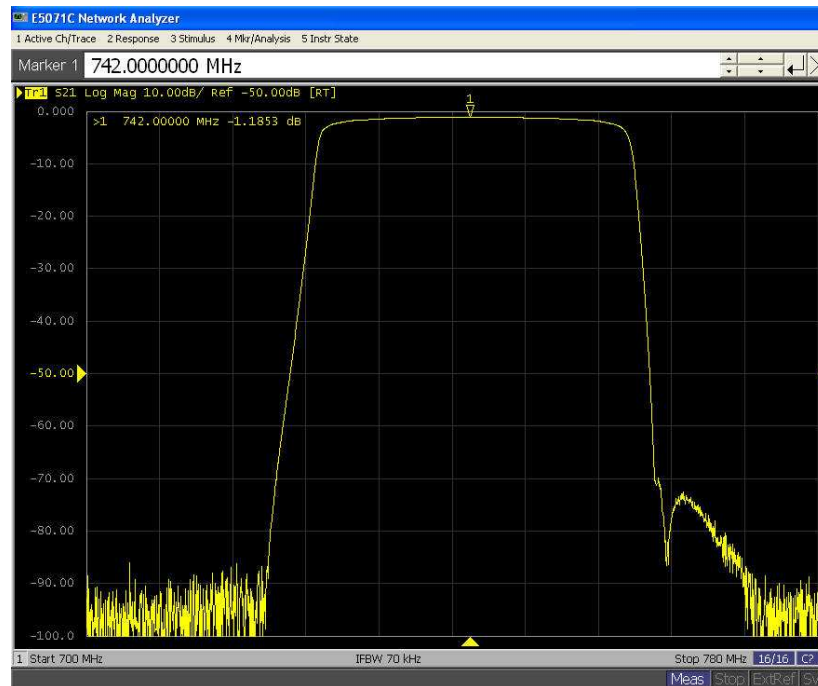
Down-link
