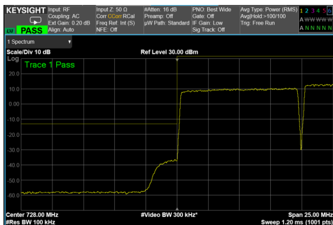
10 MHz + 5 MHz signals, Low Band Edge, 2 carriers, nominal input signal
