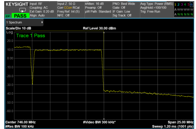
5 MHz + 10 MHz signals, High Band Edge, 2 carriers, nominal input signal + 3dB
