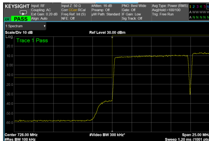
10 MHz + 5 MHz signals, Low Band Edge, 2 carriers, nominal input signal + 3dB
