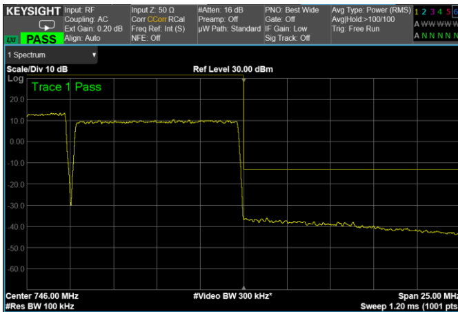
5 MHz + 10 MHz signals, High Band Edge, 2 carriers, nominal input signal
