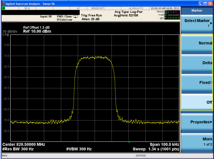
Test Data – Occupied Bandwidth 25 QAM Uplink OUTPUT
