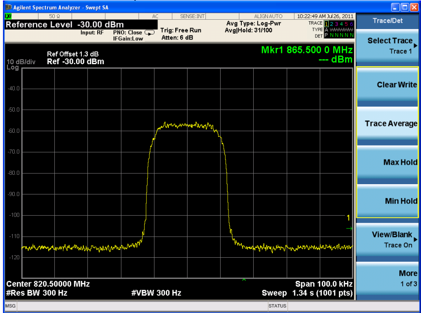
Test Data – Occupied Bandwidth 25 QAM Uplink INPUT
